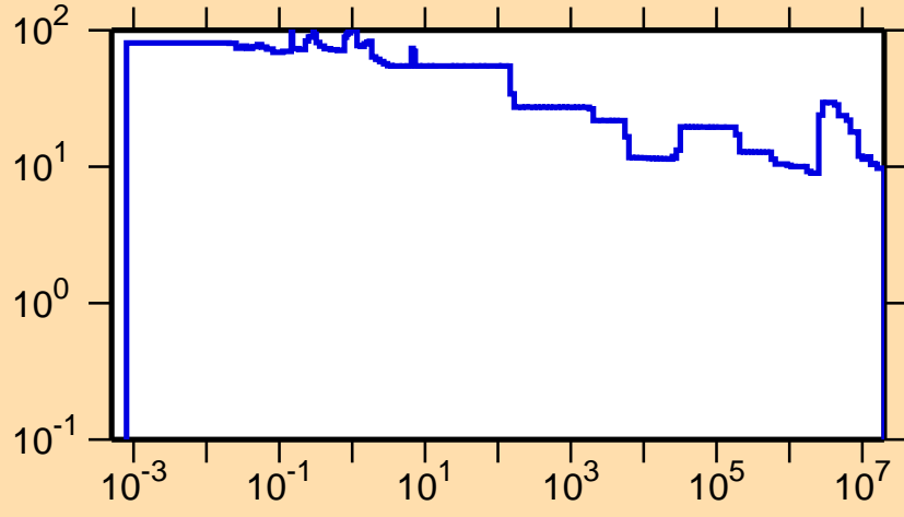
\Delta\sigma/\sigma vs. E for ^{84}\text{Y}(n,p)
