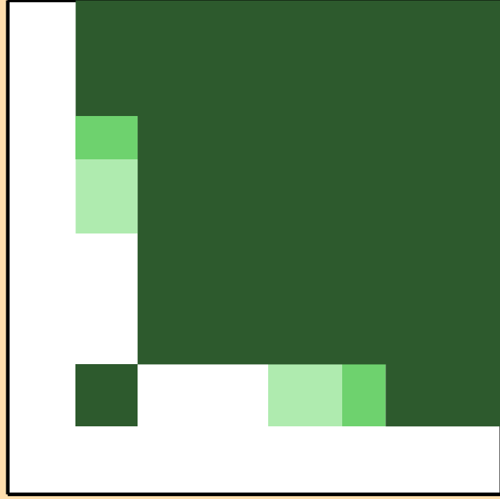
\sigma vs. E for ^{84}\text{Y}(n,\text{nd})
