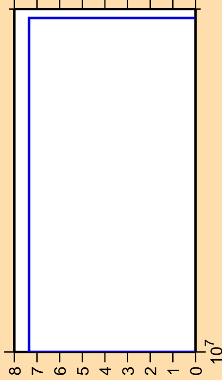
\Delta\sigma/\sigma vs. E for ^{84}\text{Y} (mt 34)
