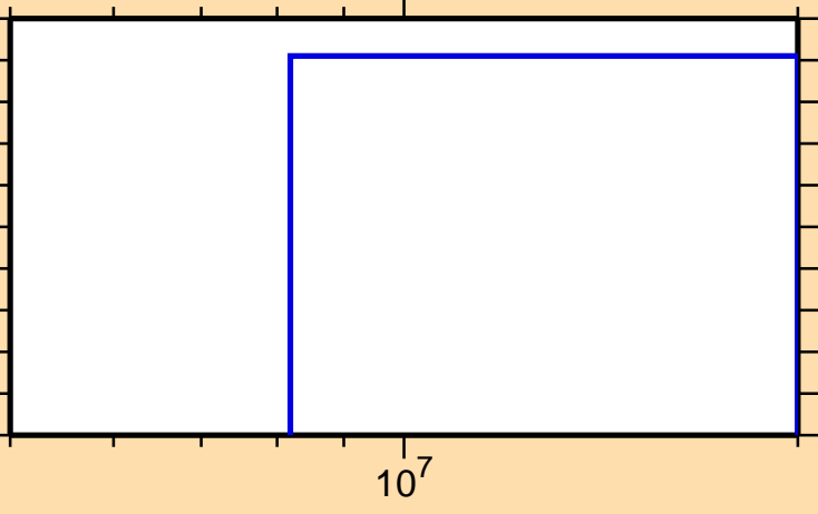
\sigma vs. E for ^{84}\text{Y}(n,\text{He}3)
