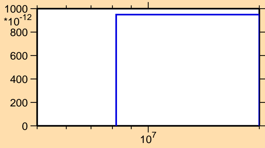
\sigma vs. E for ^{84}\text{Y}(n,\text{pt})
