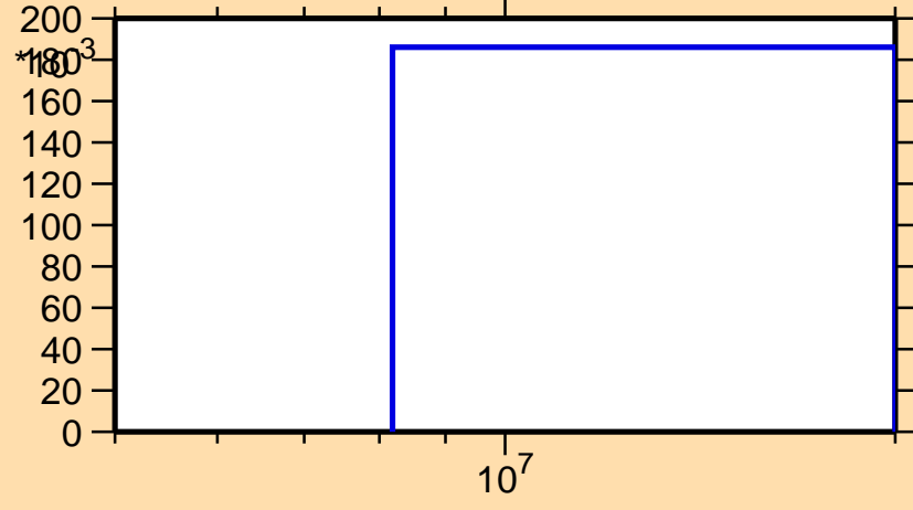
\sigma vs. E for ^{84}\text{Y}(n,2n)
