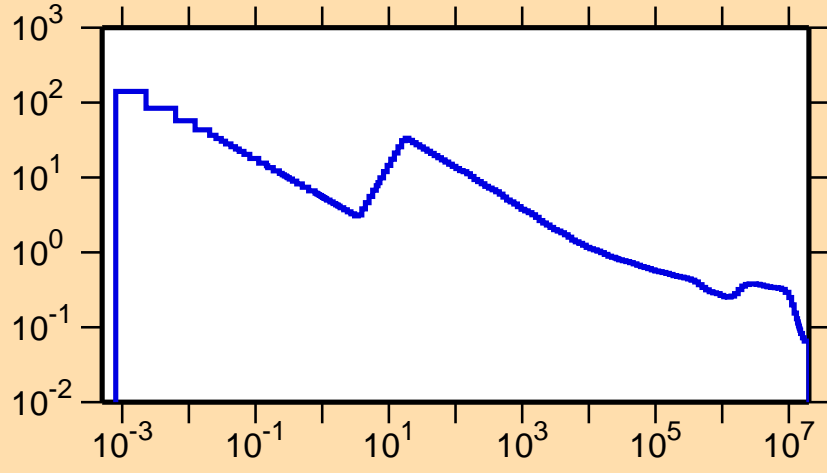
\sigma vs. E for ^{85}\text{Y}(n,p)
