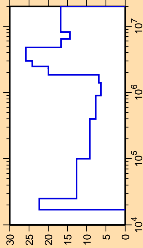
\Delta\sigma/\sigma vs. E for ^{85}\text{Y}(n,n_1)
