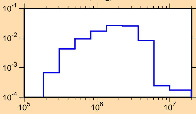
\sigma vs. E for ^{86}\text{Y}(n,n_2)
