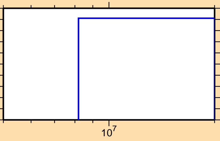
\sigma vs. E for ^{86}\text{Y}(n,2np)
