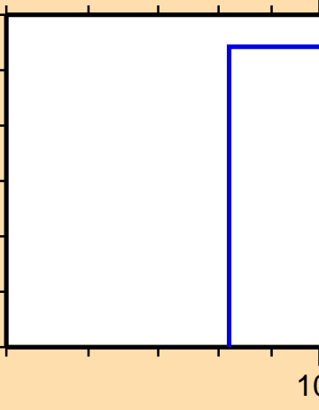
\sigma vs. E for ^{86}\text{Y}(n,nt)
