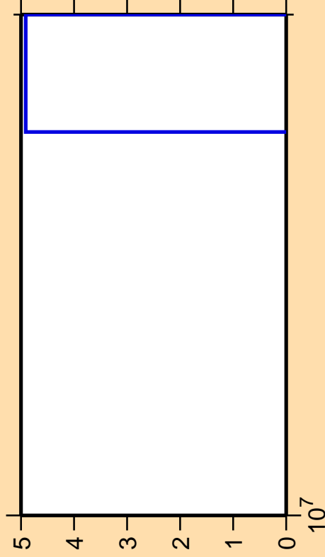
\Delta\sigma/\sigma vs. E for ^{86}\text{Y}(n,nt)
