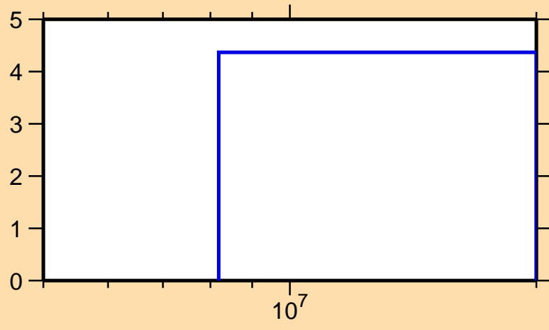
\Delta\sigma/\sigma vs. E for ^{86}\text{Y}(n,\text{el.})
