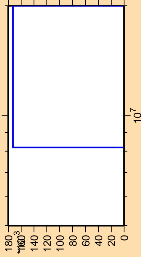
\Delta\sigma/\sigma vs. E for ^{86}\text{Y} (mt 45)
