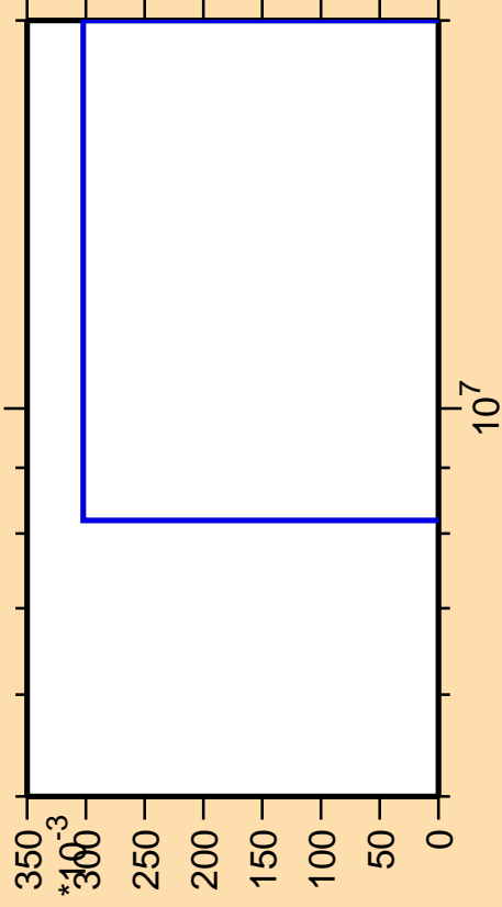
\Delta\sigma/\sigma vs. E for ^{86}\text{Y}(n,\text{pt})
