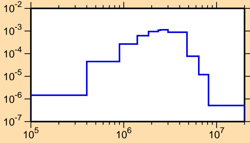
\sigma vs. E for ^{86}\text{Y}(n,n_3)
