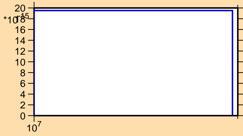
\sigma vs. E for ^{87}\text{Y}(n,nt)
