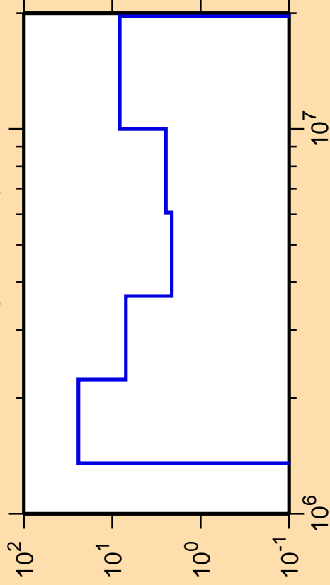
\Delta\sigma/\sigma vs. E for ^{87}\text{Y}(n,ncont.)
