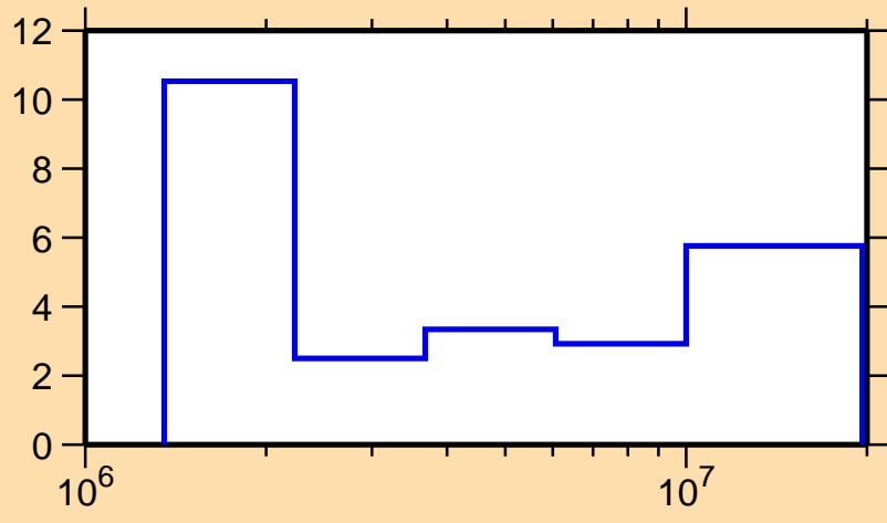
\Delta\sigma/\sigma vs. E for ^{87}\text{Y}(n,el.)
