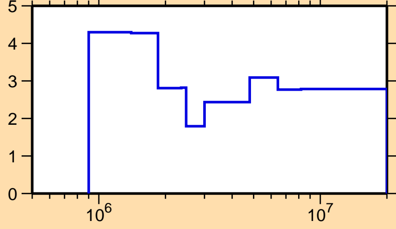
\Delta\sigma/\sigma vs. E for ^{87}\text{Y}(n,\text{nonel.})
