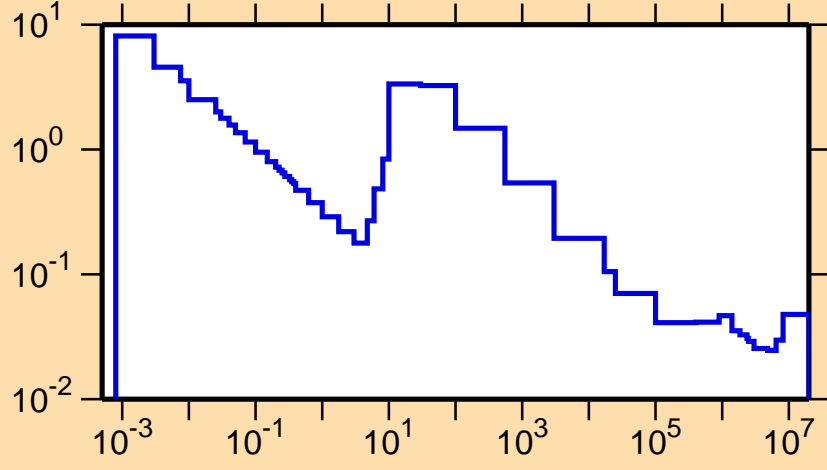
\sigma vs. E for ^{87}\text{Y}(n,p)
