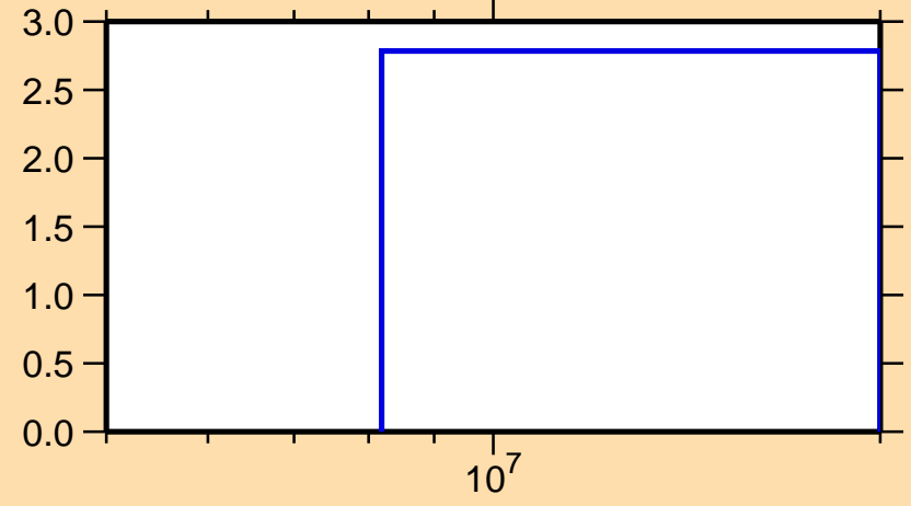
\Delta\sigma/\sigma vs. E for ^{87}\text{Y}(n,\text{nonel.})
