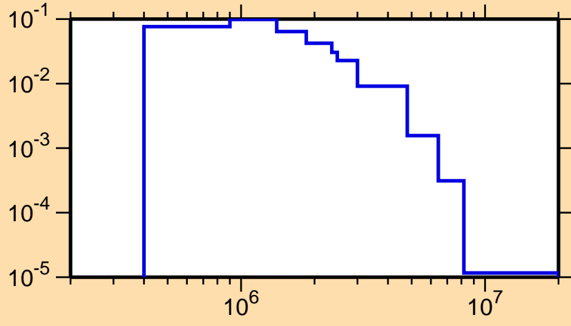
\sigma vs. E for ^{87}\text{Y}(n,n_2)
