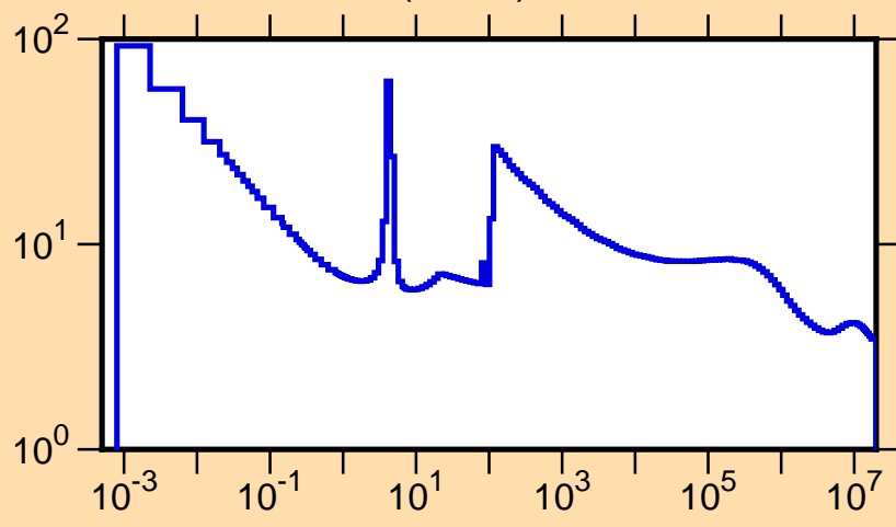
\sigma vs. E for ^{88}\text{Y}(n,\text{tot.})
