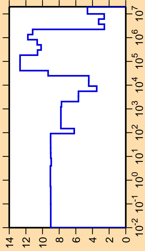
\Delta\sigma/\sigma vs. E for ^{88}\text{Y}(n,\text{el.})
