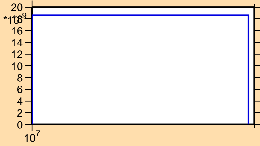
\sigma vs. E for ^{88}\text{Y}(n,\text{He}3)
