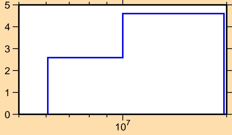
\Delta\sigma/\sigma vs. E for ^{88}\text{Y}(n,\text{el.})
