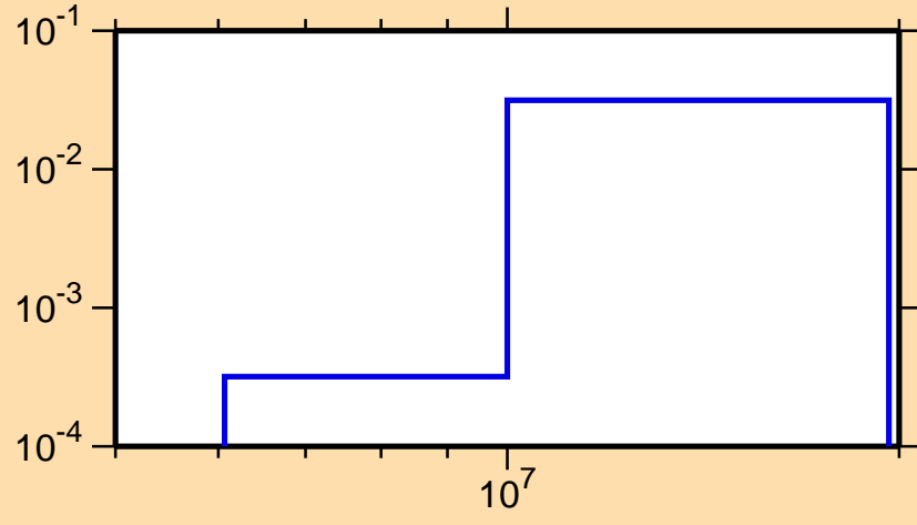
\sigma vs. E for ^{88}\text{Y}(n,np)
