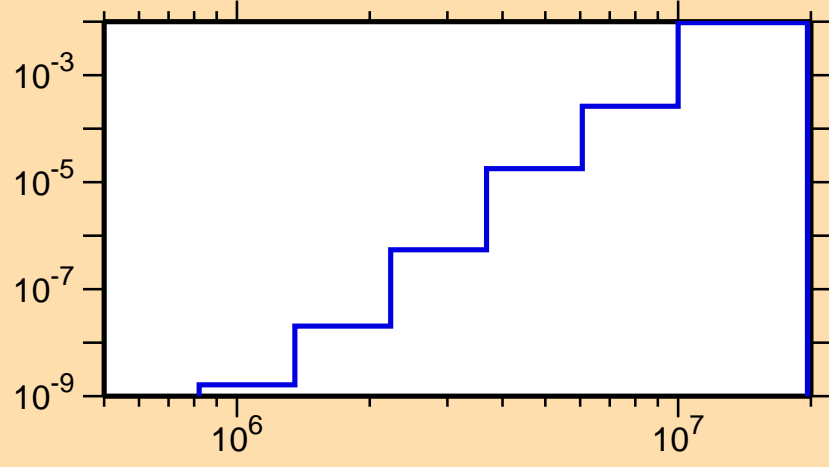
\sigma vs. E for ^{88}\text{Y}(n,\alpha)
