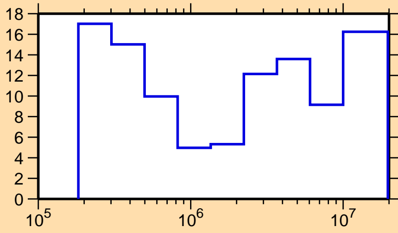
\Delta\sigma/\sigma vs. E for ^{88}\text{Y}(n,n_1)
