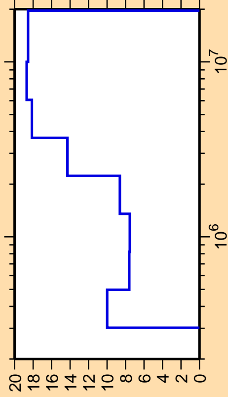
\Delta\sigma/\sigma vs. E for ^{88}\text{Y}(n,n_2)
