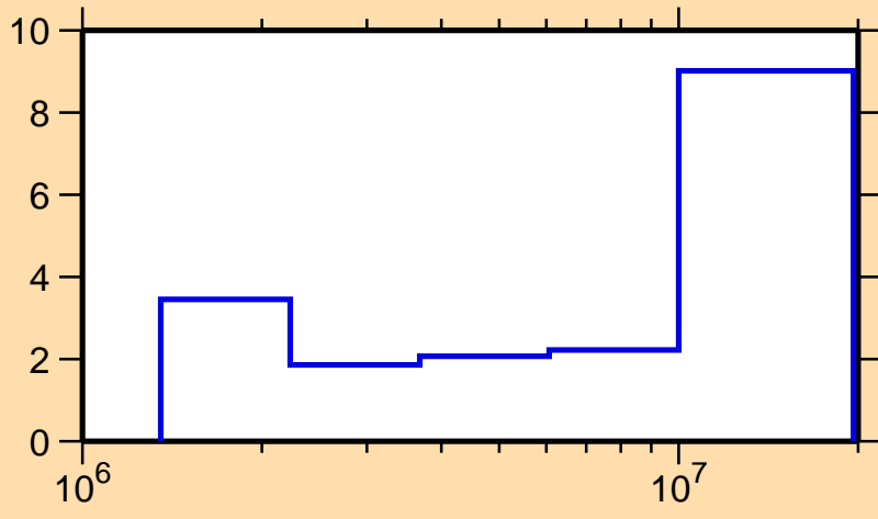
\Delta\sigma/\sigma vs. E for ^{88}\text{Y}(n,\text{inel.})
