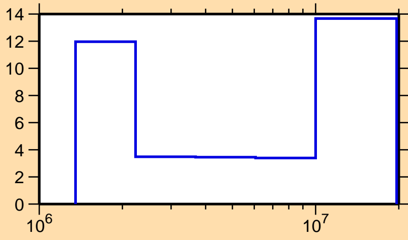
\Delta\sigma/\sigma vs. E for ^{88}\text{Y}(n,n\text{cont.})
