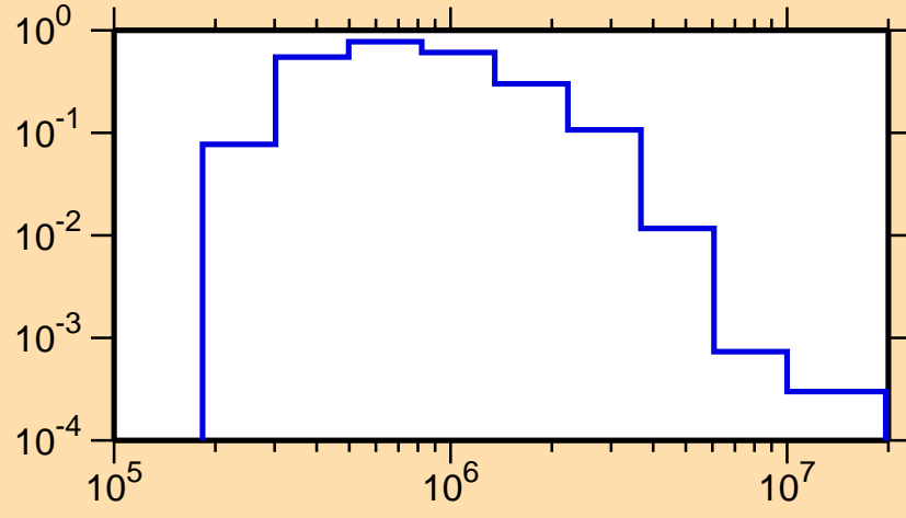
\sigma vs. E for ^{88}\text{Y}(n,n_1)
