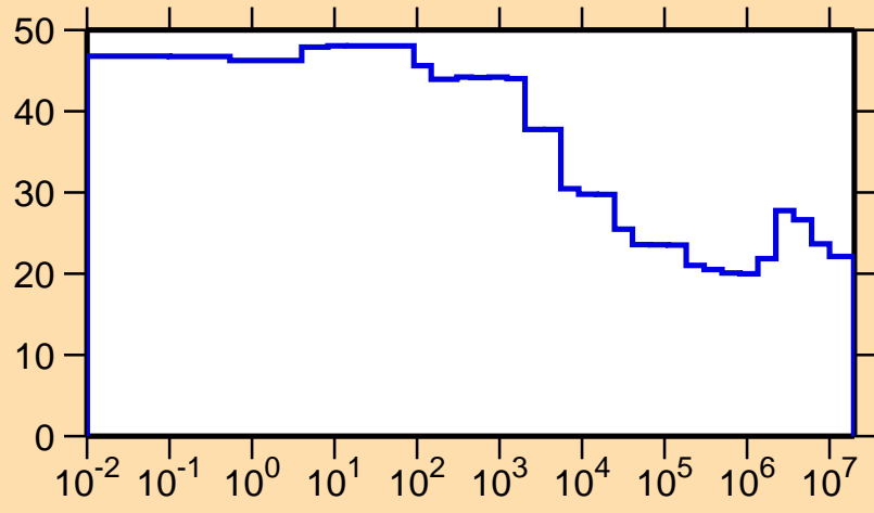
\Delta\sigma/\sigma vs. E for ^{88}\text{Y}(n,p)
