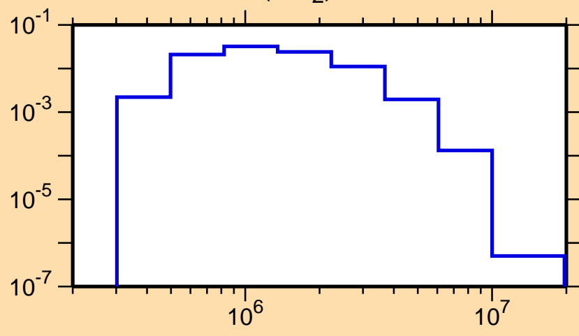
\sigma vs. E for ^{88}\text{Y}(n,n_2)
