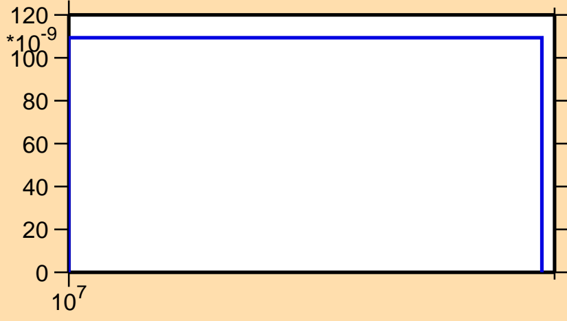
\sigma vs. E for ^{88}\text{Y}(n,\text{nd})
