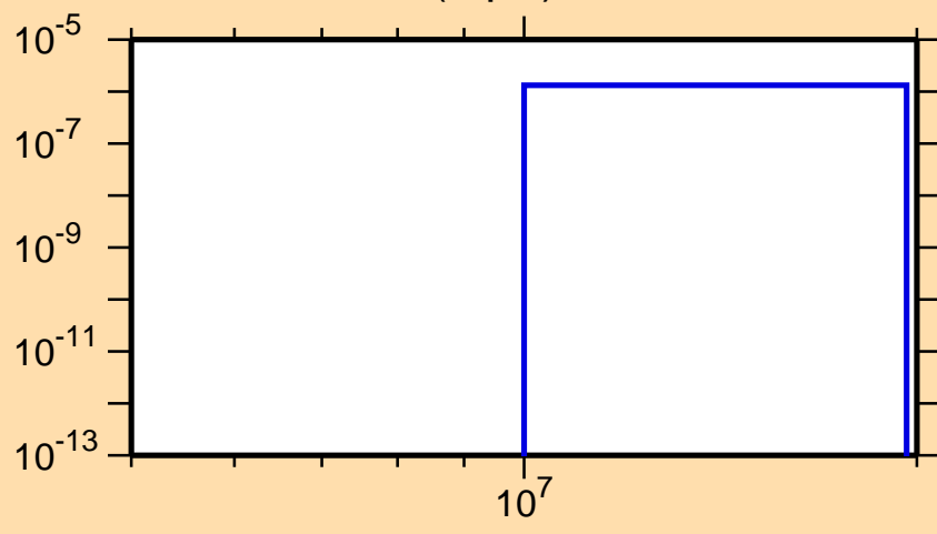
\sigma vs. E for ^{88}\text{Y}(n,p\alpha)
