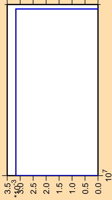
\Delta\sigma/\sigma vs. E for ^{88}\text{Y}(n,pd)
