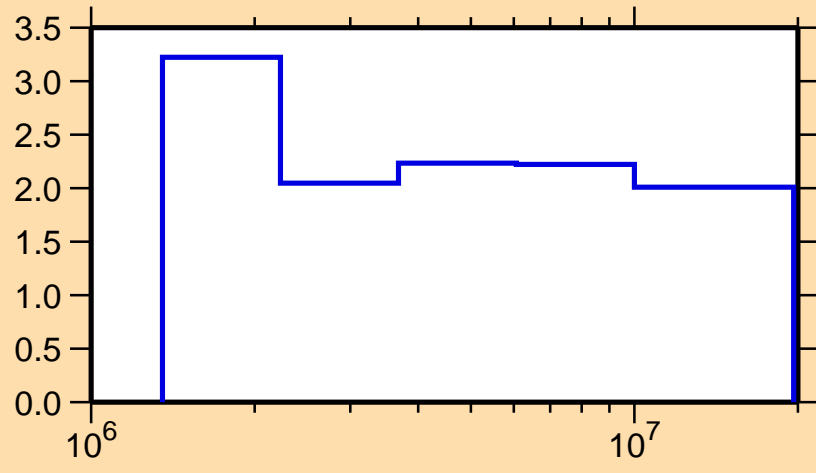
\Delta\sigma/\sigma vs. E for ^{88}\text{Y}(n,n\text{onel.})
