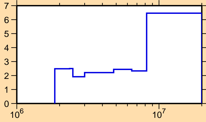
\Delta\sigma/\sigma vs. E for ^{88}\text{Y}(n,\text{inel.})
