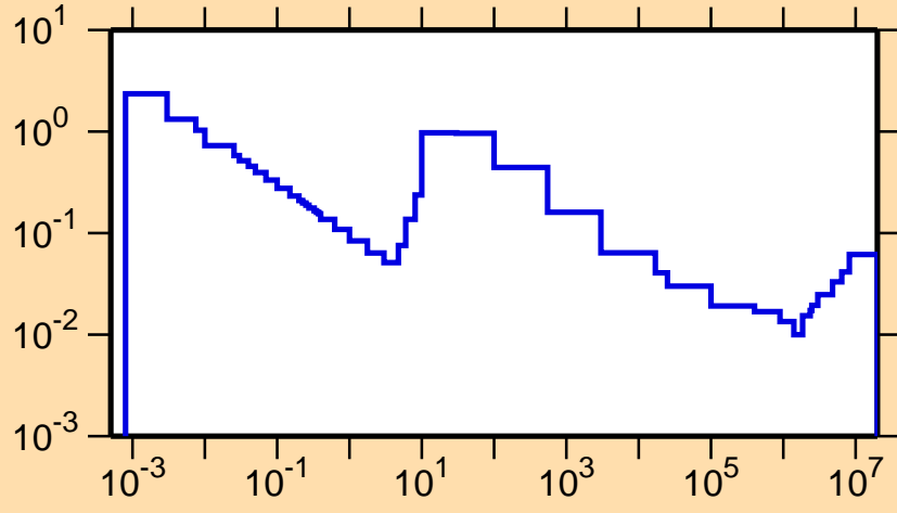
\sigma vs. E for ^{88}\text{Y}(n,p)
