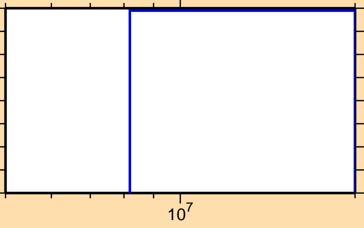
\sigma vs. E for ^{88}\text{Y}(n,\text{He}3)
