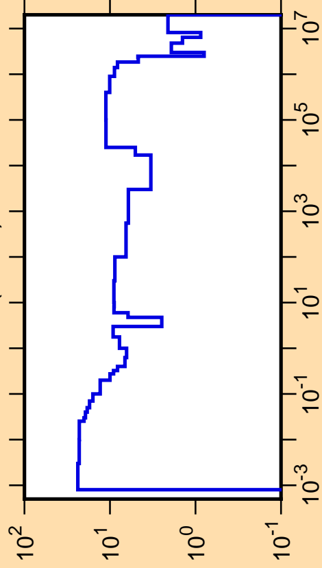
\Delta\sigma/\sigma vs. E for ^{88}\text{Y}(n,\text{tot.})
