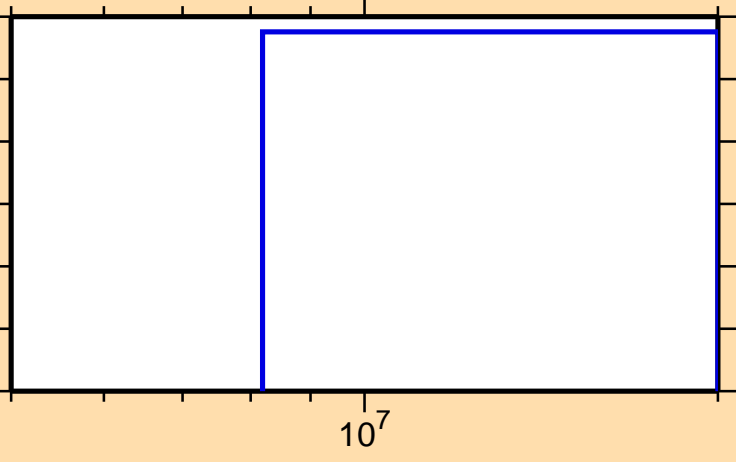
\sigma vs. E for ^{88}\text{Y}(n,n\alpha)
