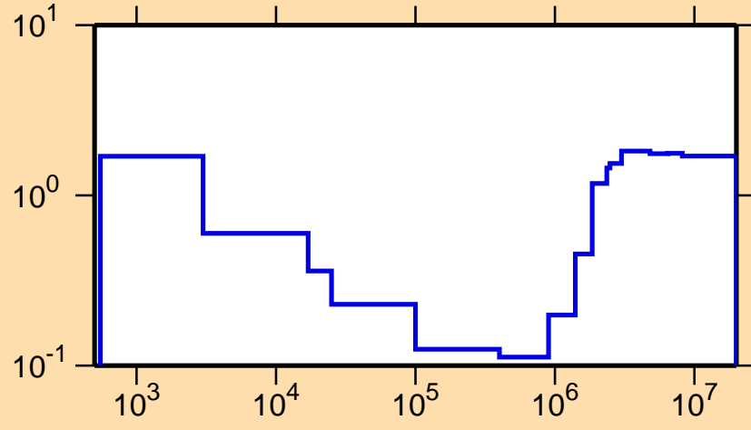
\sigma vs. E for ^{89}\text{Y}(n,\text{nonel.})
