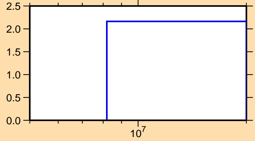
\Delta\sigma/\sigma vs. E for ^{89}\text{Y}(n,\text{el.})
