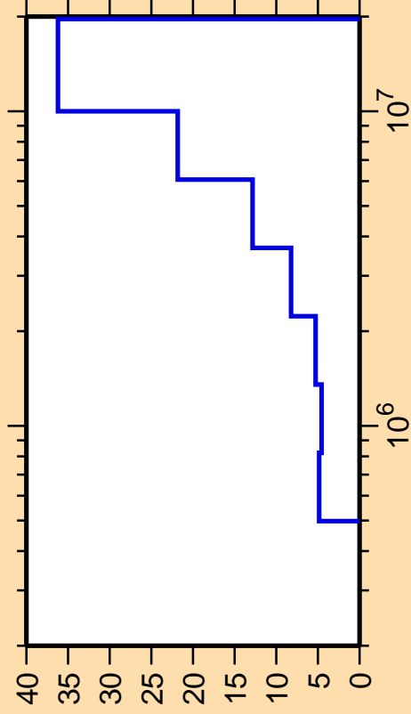
\Delta\sigma/\sigma vs. E for ^{90}\text{Y}(n,n_2)
