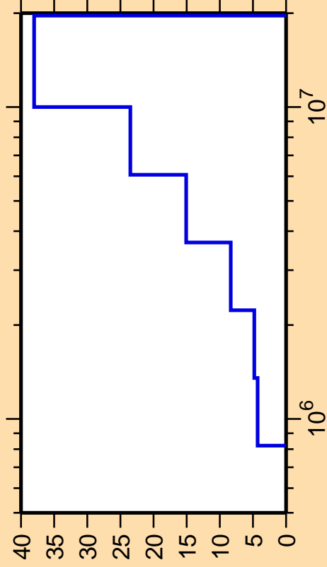
\Delta\sigma/\sigma vs. E for ^{90}\text{Y}(n,n_4)
