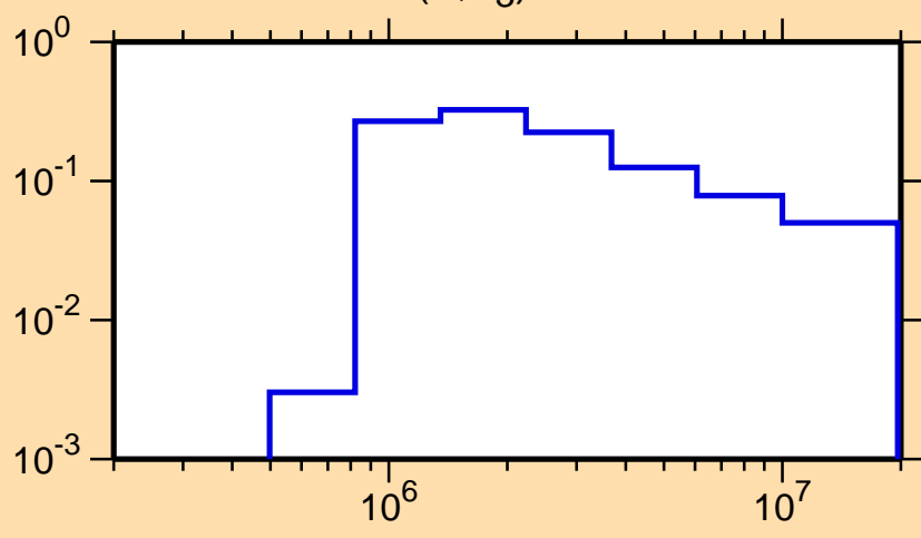
\sigma vs. E for ^{90}\text{Y}(n,n_3)
