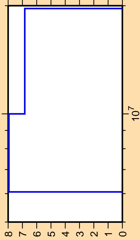
\Delta\sigma/\sigma vs. E for ^{90}\text{Y}(n,2n)
