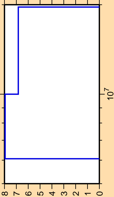
\Delta\sigma/\sigma vs. E for ^{90}\text{Y}(n,2n)
