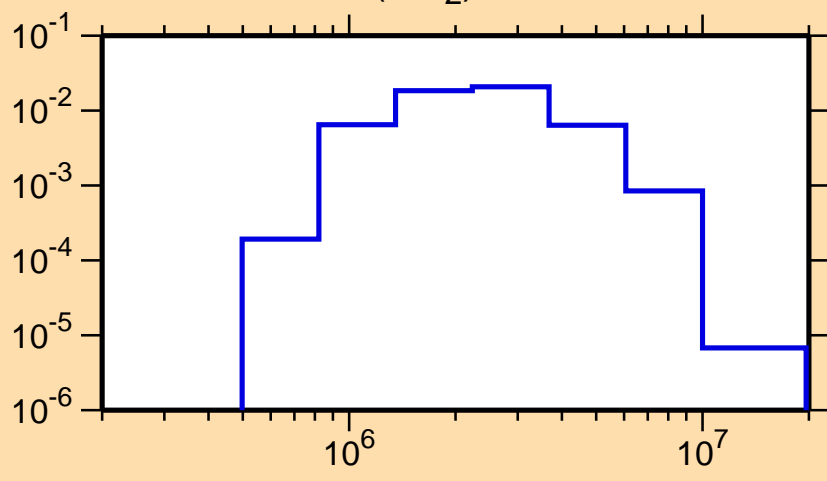
\sigma vs. E for ^{90}\text{Y}(n,n_2)
