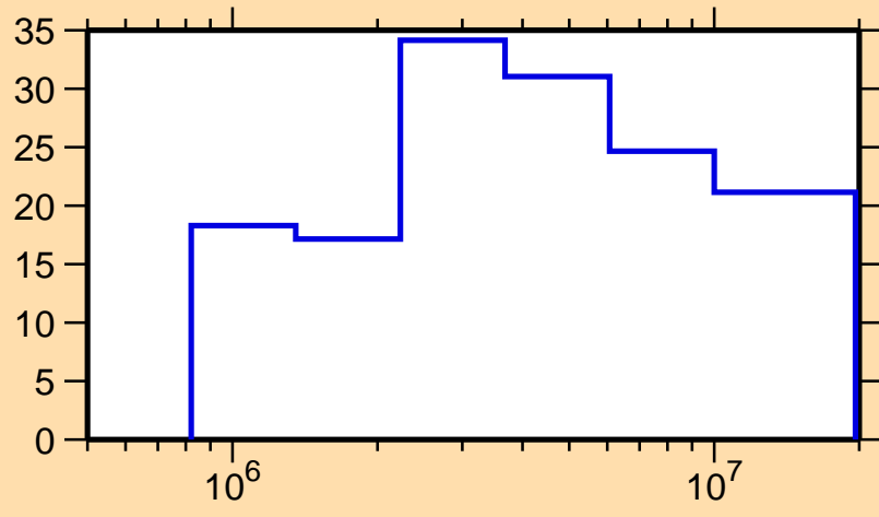
\Delta\sigma/\sigma vs. E for ^{90}\text{Y}(n,p)
