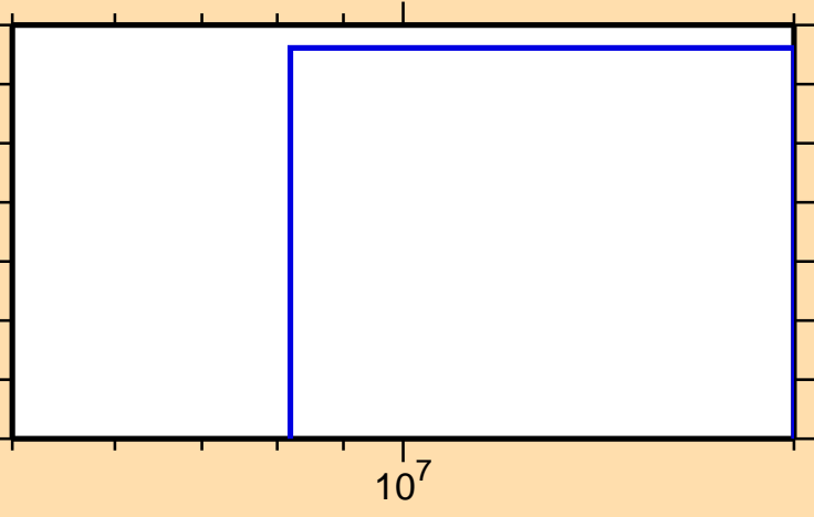
\sigma vs. E for ^{90}\text{Y}(n,\text{nd})
