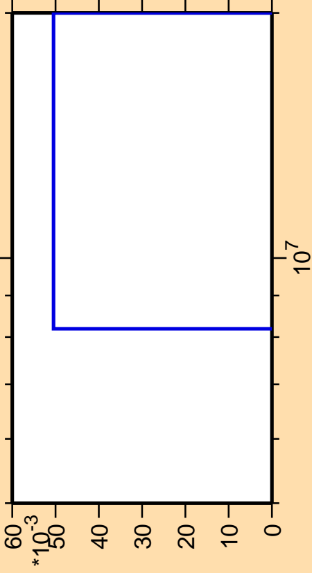
\Delta\sigma/\sigma vs. E for ^{90}\text{Y}(n,2n\alpha)
