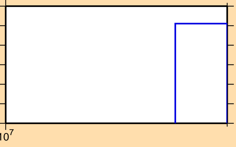
\sigma vs. E for ^{91}\text{Y} (mt 34)
