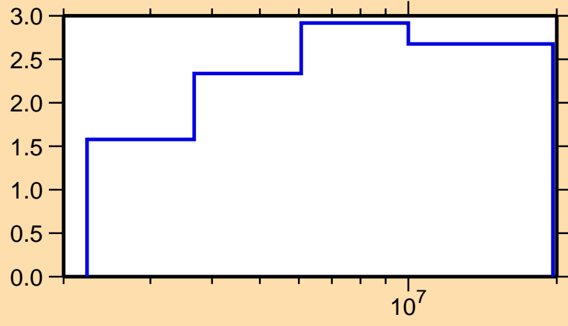
\Delta\sigma/\sigma vs. E for ^{91}\text{Y}(n,n\text{onel.})
