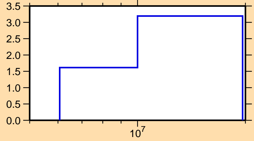
\Delta\sigma/\sigma vs. E for ^{91}\text{Y}(n,\text{el.})
