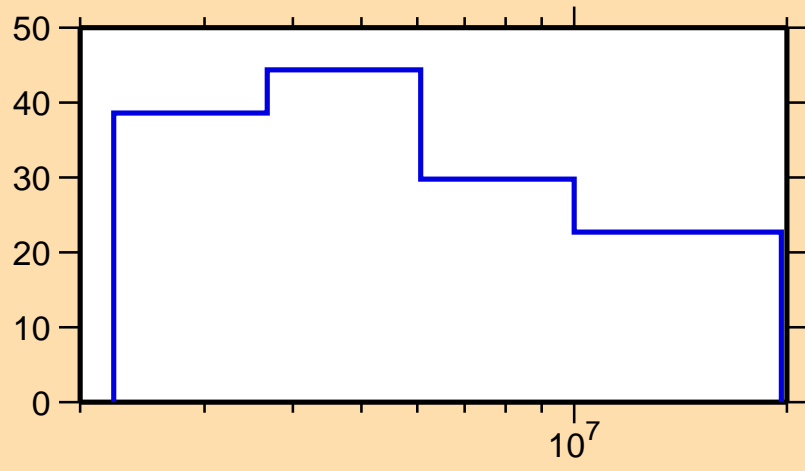
\Delta\sigma/\sigma vs. E for ^{91}\text{Y}(n,p)
