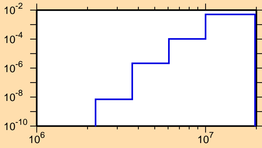
\sigma vs. E for ^{91}\text{Y}(n,\alpha)
