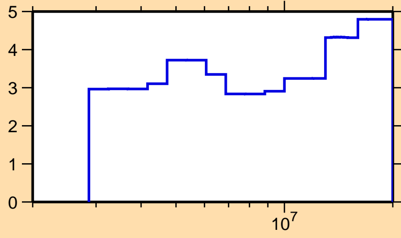
\Delta\sigma/\sigma vs. E for ^{92}\text{Y}(n,\text{el.})
