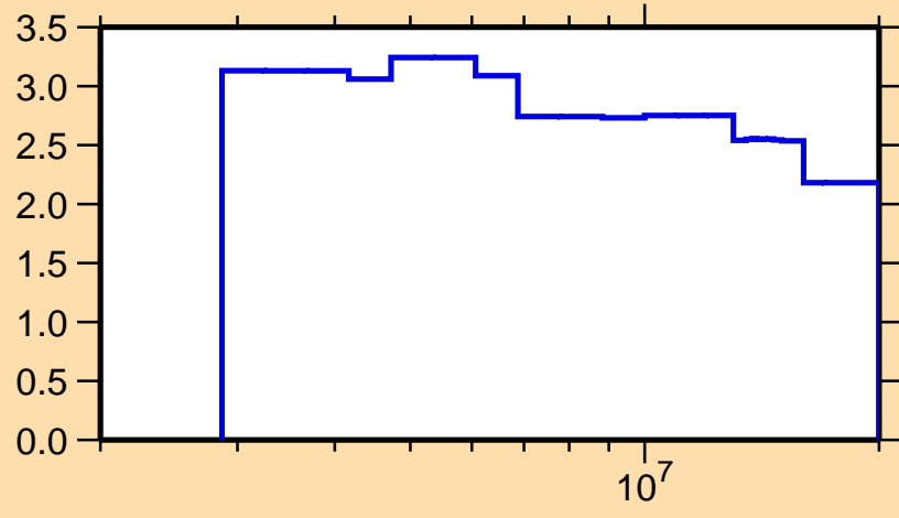
\Delta\sigma/\sigma vs. E for ^{92}\text{Y}(n,n\text{onel.})
