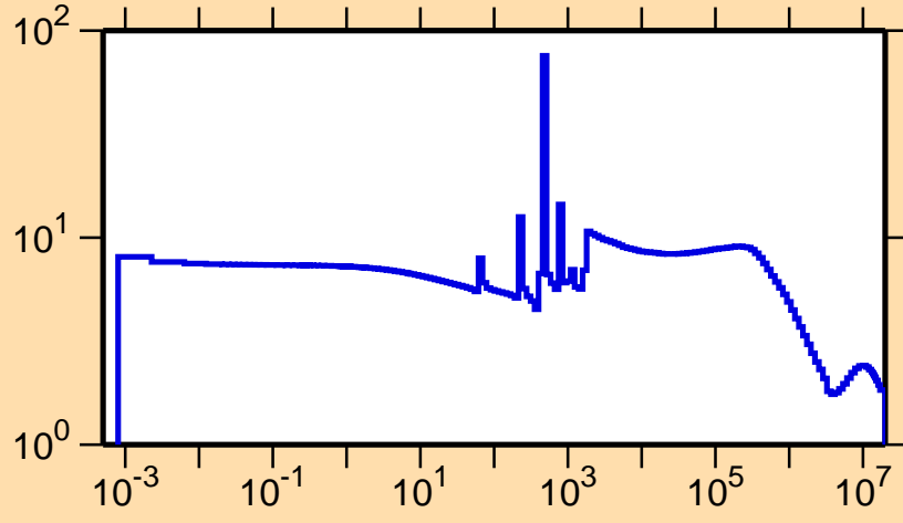
\sigma vs. E for ^{92}\text{Y}(n,\text{el.})
