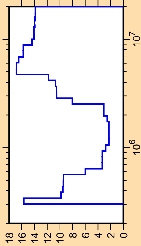
\Delta\sigma/\sigma vs. E for ^{92}\text{Y}(n,n_2)
