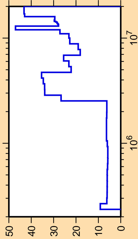
\Delta\sigma/\sigma vs. E for ^{92}\text{Y}(n,n_1)
