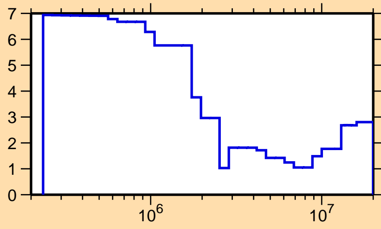
\Delta\sigma/\sigma vs. E for ^{92}\text{Y}(n,\text{tot.})
