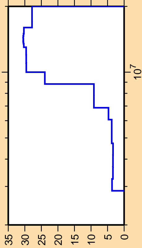
\Delta\sigma/\sigma vs. E for ^{92}\text{Y}(n,\text{ncont.})
