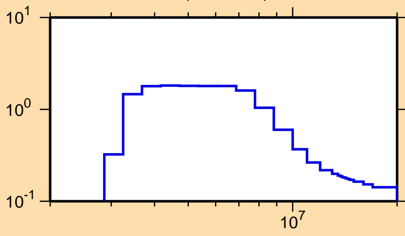
\sigma vs. E for ^{92}\text{Y}(n,n\text{cont.})
