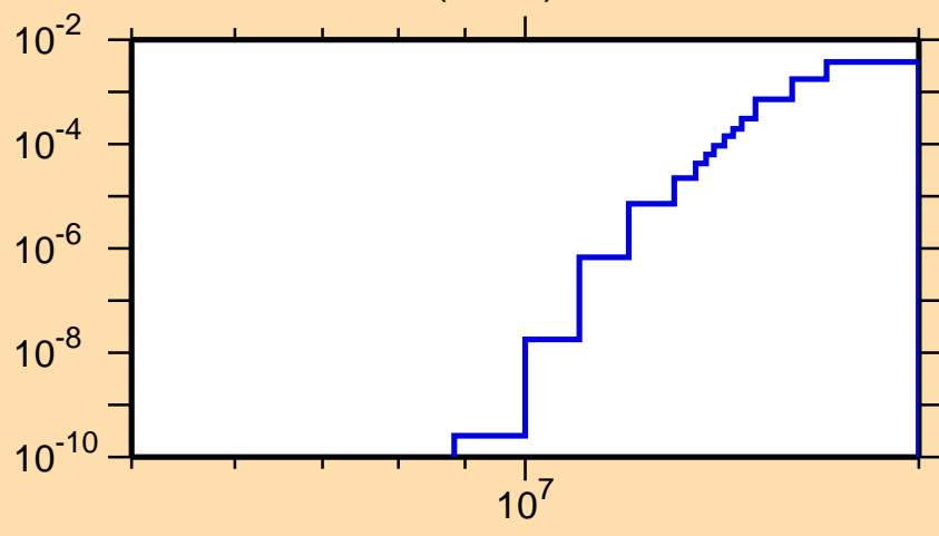
\sigma vs. E for ^{92}\text{Y}(n,n\alpha)
