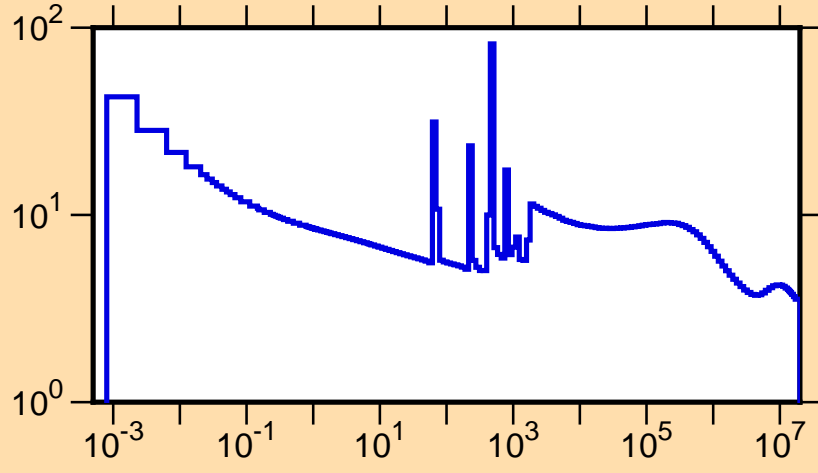
\sigma vs. E for ^{92}\text{Y}(n,\text{tot.})
