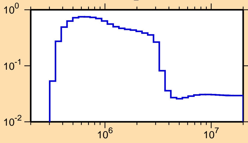
\sigma vs. E for ^{92}\text{Y}(n,n_2)
