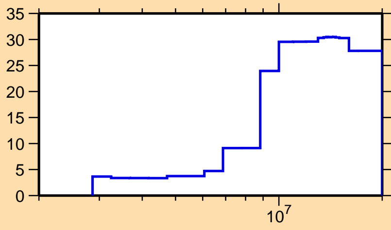
\Delta\sigma/\sigma vs. E for ^{92}\text{Y}(n,n\text{cont.})
