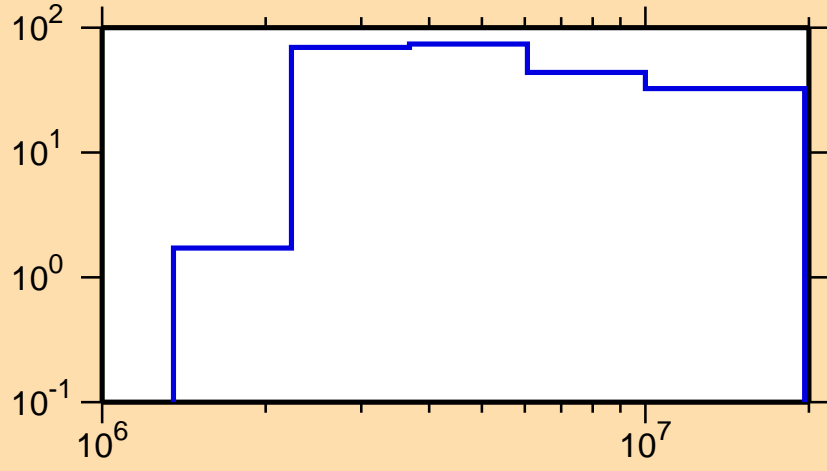
\Delta\sigma/\sigma vs. E for ^{92}\text{Y}(n,p)
