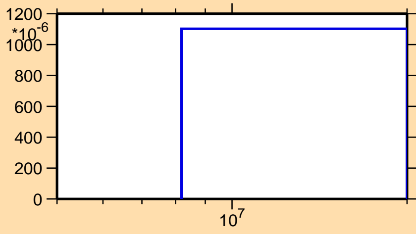
\sigma vs. E for ^{92}\text{Y}(n,np)
