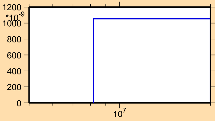
\sigma vs. E for ^{92}\text{Y}(n,\text{nd})
