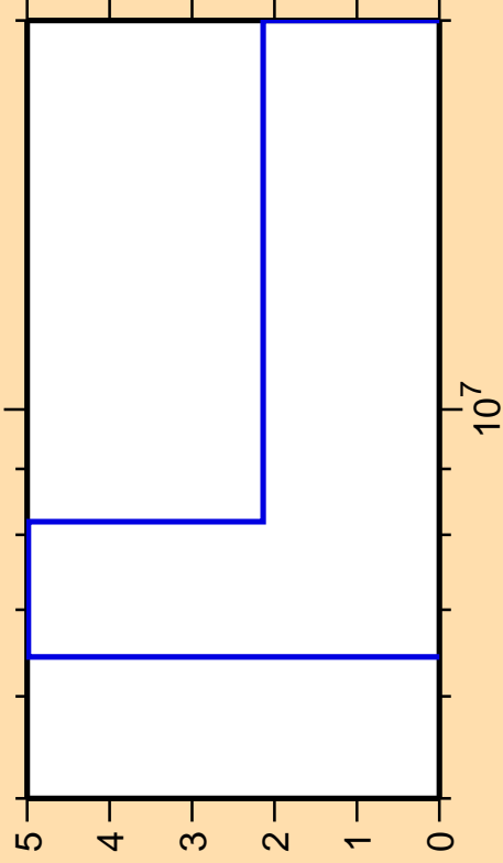
\Delta\sigma/\sigma vs. E for ^{92}\text{Y}(n,2n)
