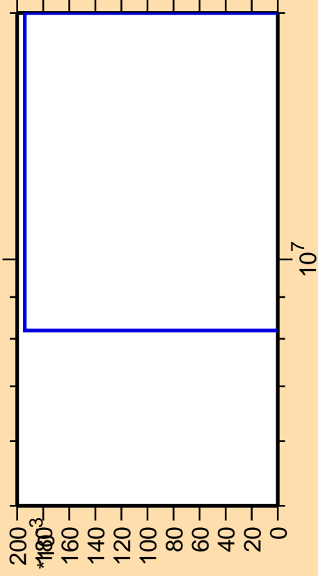
\Delta\sigma/\sigma vs. E for ^{92}\text{Y}(n,p\alpha)
