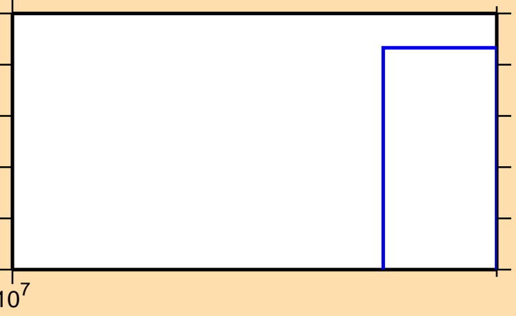
\sigma vs. E for ^{93}\text{Y} (mt 11)
