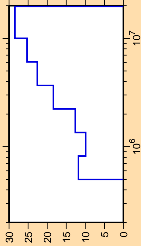
\Delta\sigma/\sigma vs. E for ^{93}\text{Y}(n,n_2)
