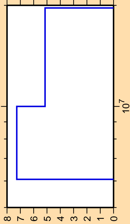
\Delta\sigma/\sigma vs. E for ^{93}\text{Y}(n,2n)
