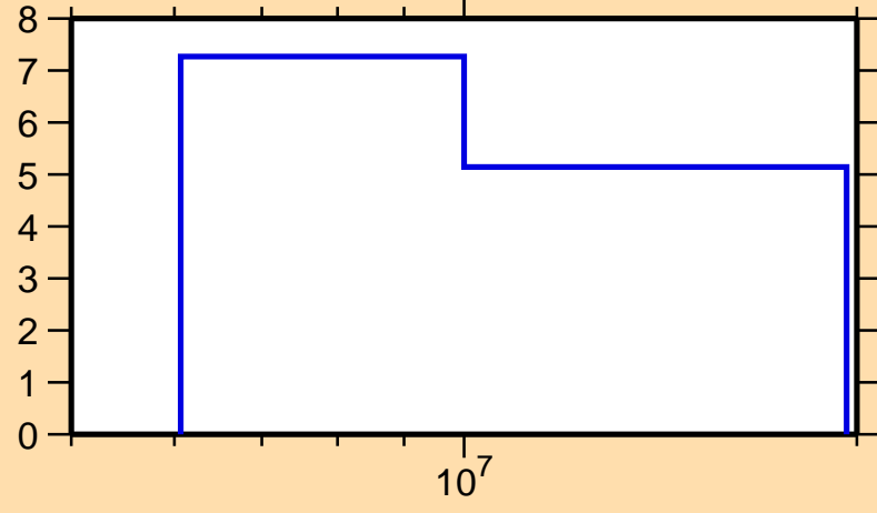
\Delta\sigma/\sigma vs. E for ^{93}\text{Y}(n,2n)
