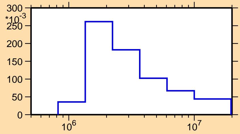
\sigma vs. E for ^{93}\text{Y}(n,n_4)
