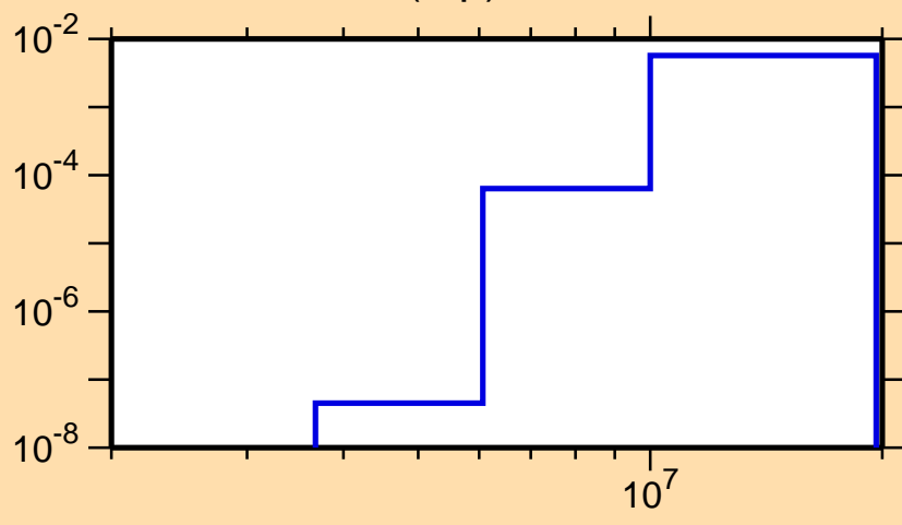
\sigma vs. E for ^{93}\text{Y}(n,p)
