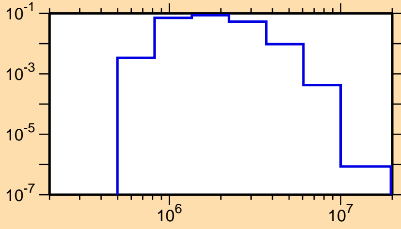
\sigma vs. E for ^{93}\text{Y}(n,n_2)
