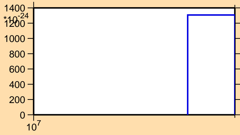
\sigma vs. E for ^{94}\text{Y}(n,3n\alpha)
