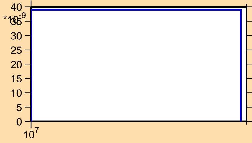
\sigma vs. E for ^{94}\text{Y}(n,nt)
