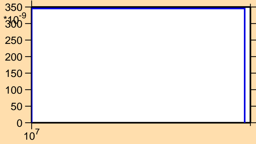
\sigma vs. E for ^{94}\text{Y}(n,\text{nd})
