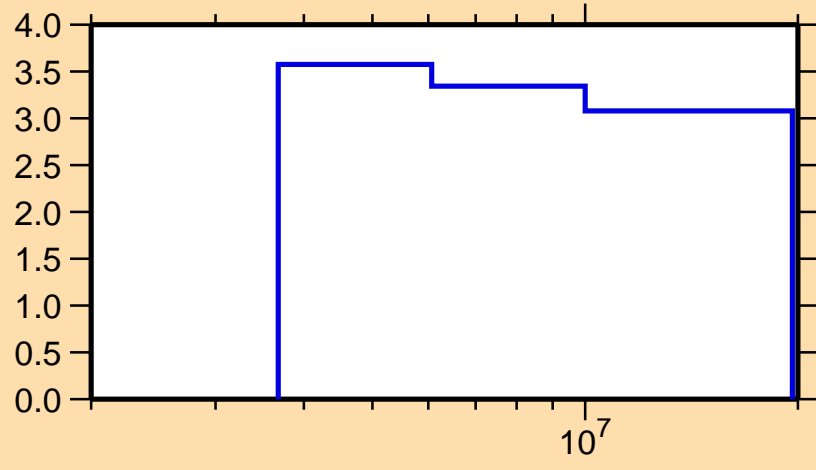
\Delta\sigma/\sigma vs. E for ^{94}\text{Y}(n,n\text{onel.})
