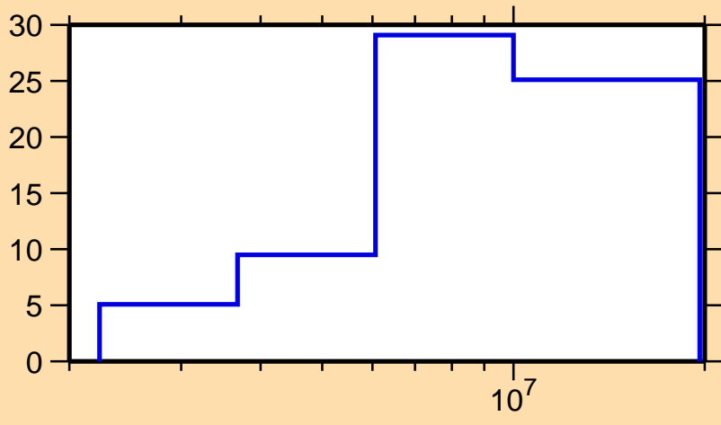
\Delta\sigma/\sigma vs. E for ^{94}\text{Y}(n,n_1)
