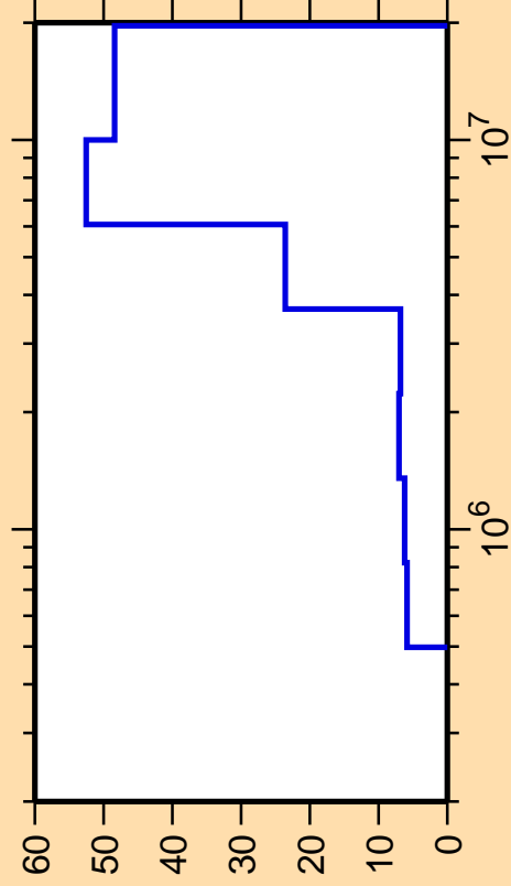
\Delta\sigma/\sigma vs. E for ^{94}\text{Y}(n,n_2)
