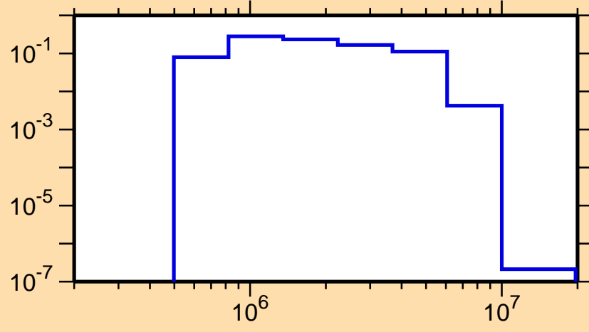
\sigma vs. E for ^{94}\text{Y}(n,n_2)
