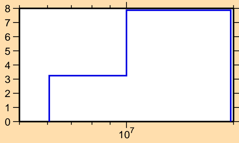
\Delta\sigma/\sigma vs. E for ^{94}\text{Y}(n,\text{el.})
