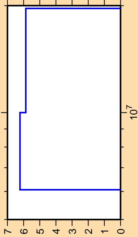
\Delta\sigma/\sigma vs. E for ^{94}\text{Y}(n,2n)
