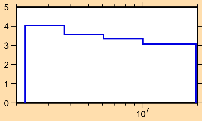
\Delta\sigma/\sigma vs. E for ^{94}\text{Y}(n,\text{nonel.})
