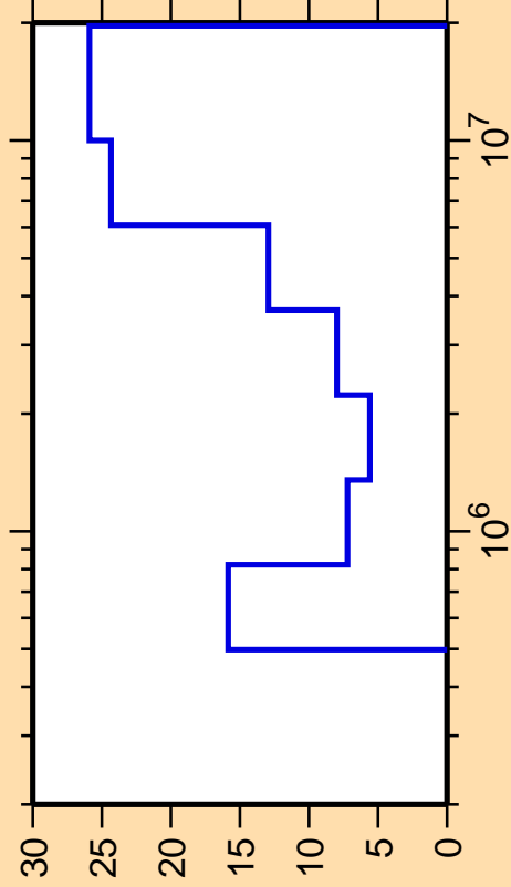
\Delta\sigma/\sigma vs. E for ^{94}\text{Y}(n,n_3)
