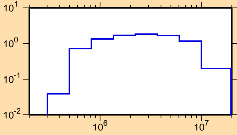
\sigma vs. E for ^{94}\text{Y}(n,\text{inel.})
