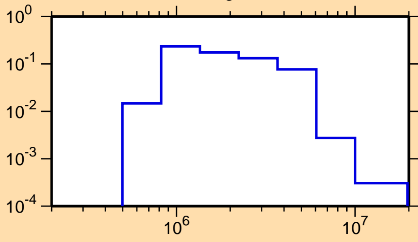
\sigma vs. E for ^{94}\text{Y}(n,n_3)
