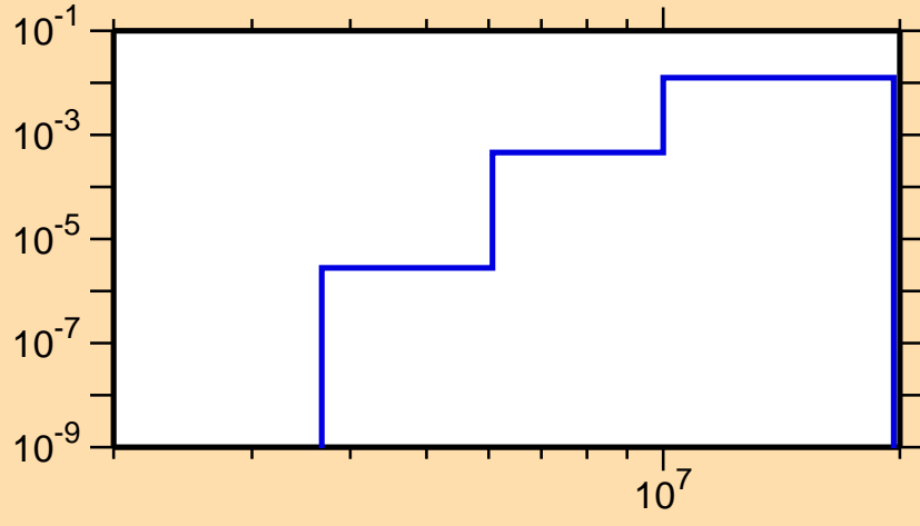
\sigma vs. E for ^{94}\text{Y}(n,p)
