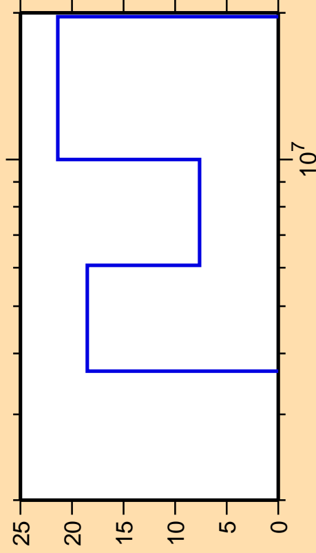
\Delta\sigma/\sigma vs. E for ^{94}\text{Y}(n,n\text{cont.})
