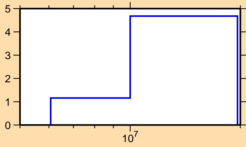
\Delta\sigma/\sigma vs. E for ^{94}\text{Y}(n,\text{tot.})
