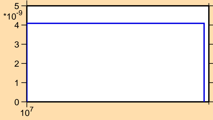
\sigma vs. E for ^{94}\text{Y}(n,2np)
