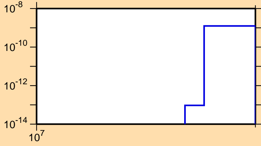
\sigma vs. E for ^{95}\text{Y}(n,2n\alpha)
