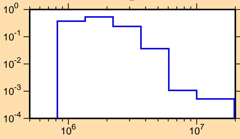
\sigma vs. E for ^{95}\text{Y}(n,n_2)
