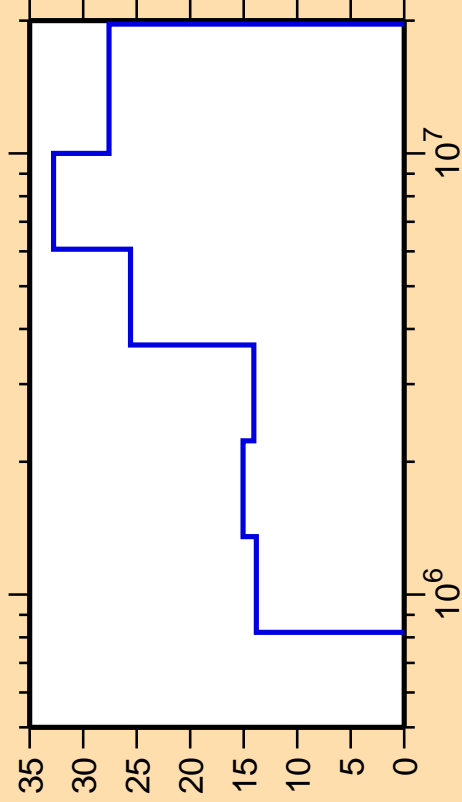
\Delta\sigma/\sigma vs. E for ^{95}\text{Y}(n,n_2)
