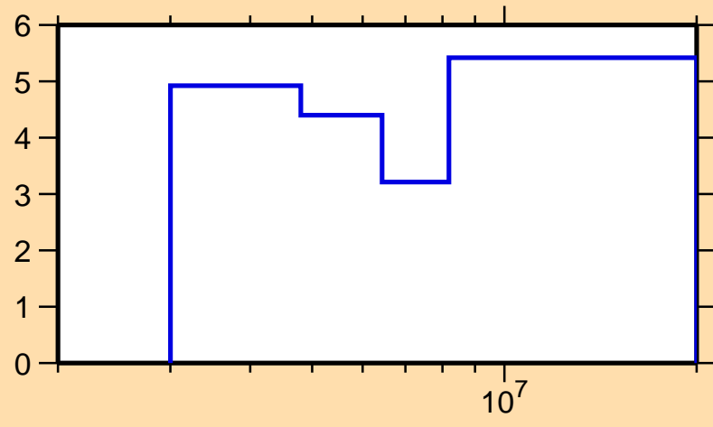
\Delta\sigma/\sigma vs. E for ^{95}\text{Y}(n,\text{tot.})
