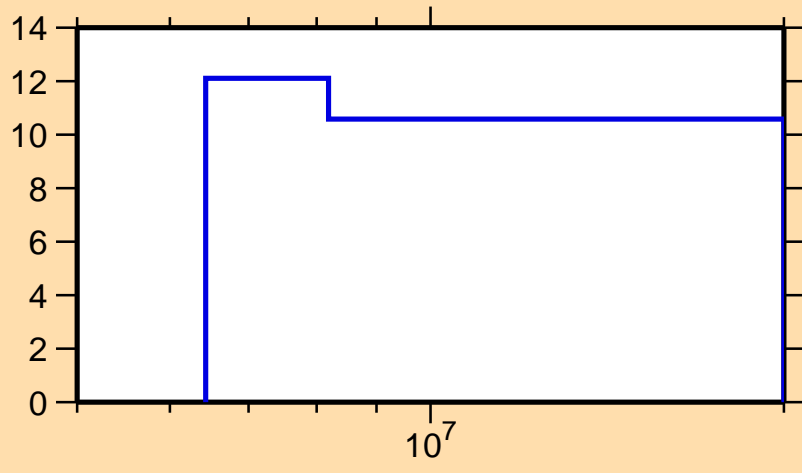
\Delta\sigma/\sigma vs. E for ^{95}\text{Y}(n,2n)
