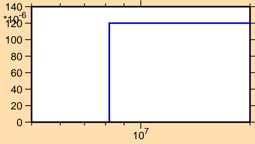
\sigma vs. E for ^{95}\text{Y}(n,np)
