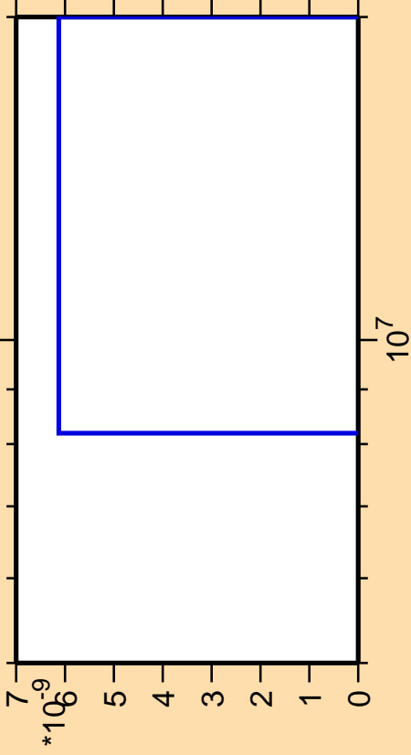
\Delta\sigma/\sigma vs. E for ^{95}\text{Y}(n,3n\alpha)
