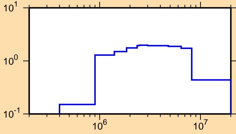
\sigma vs. E for ^{95}\text{Y}(n,\text{inel.})
