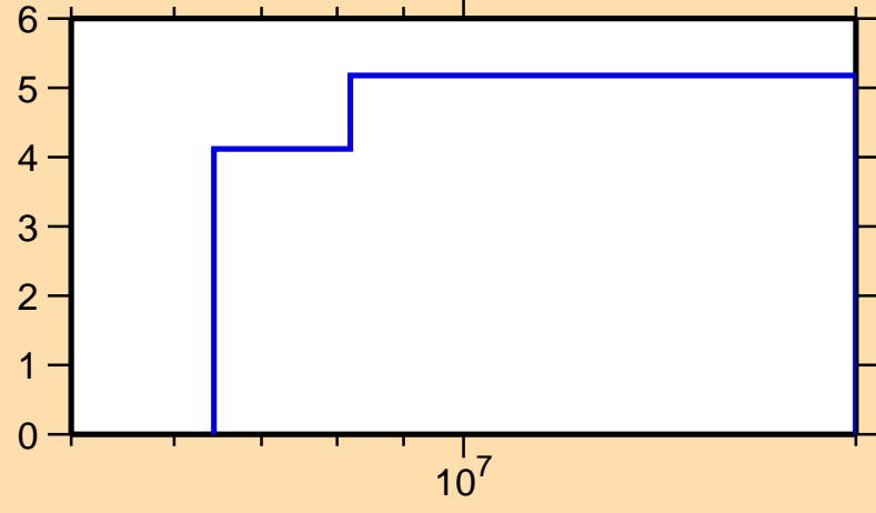
\Delta\sigma/\sigma vs. E for ^{95}\text{Y}(n,\text{el.})
