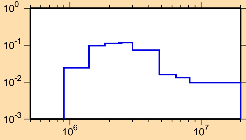
\sigma vs. E for ^{95}\text{Y}(n,n_3)
