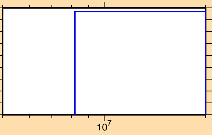
\sigma vs. E for ^{95}\text{Y}(n,n\alpha)
