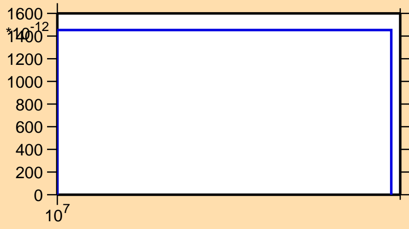
\sigma vs. E for ^{96}\text{Y}(n,2n\alpha)
