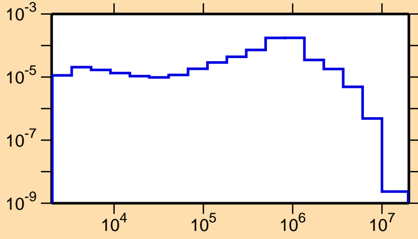
\sigma vs. E for ^{96}\text{Y}(n,n_2)
