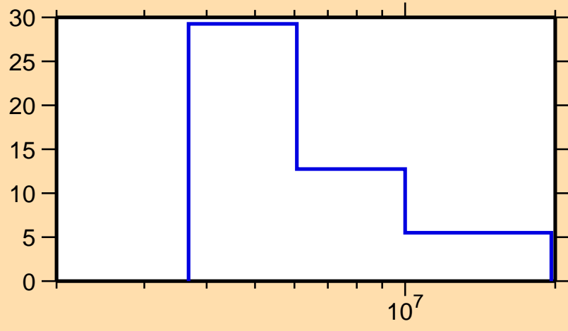
\Delta\sigma/\sigma vs. E for ^{96}\text{Y}(n,2n)
