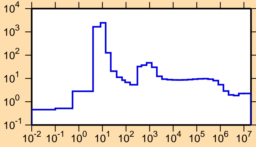
\sigma vs. E for ^{96}\text{Y}(n,\text{el.})
