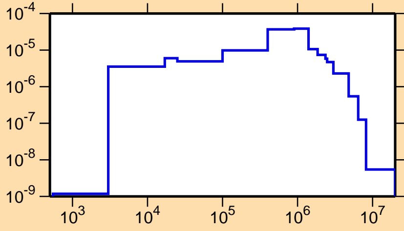
\sigma vs. E for ^{96}\text{Y}(n,n_1)
