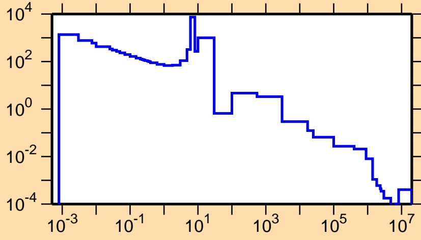
\sigma vs. E for ^{96}\text{Y}(n,\gamma)
