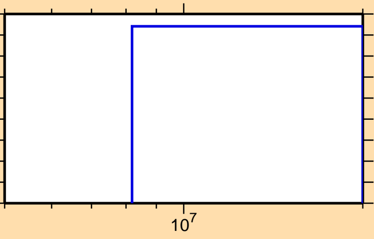
\sigma vs. E for ^{96}\text{Y}(n,np)
