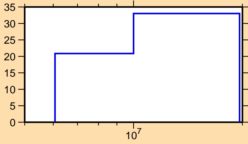
\Delta\sigma/\sigma vs. E for ^{97}\text{Y}(n,n\text{cont.})
