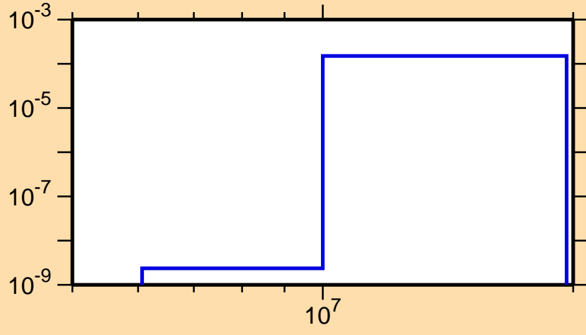
\sigma vs. E for ^{97}\text{Y}(n,\alpha)
