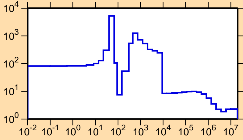
\sigma vs. E for ^{97}\text{Y}(n,\text{el.})
