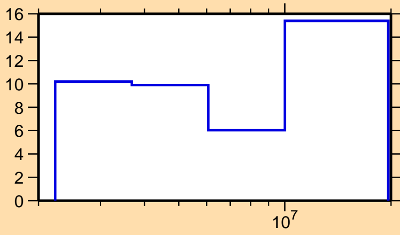
\Delta\sigma/\sigma vs. E for ^{97}\text{Y}(n,el.)
