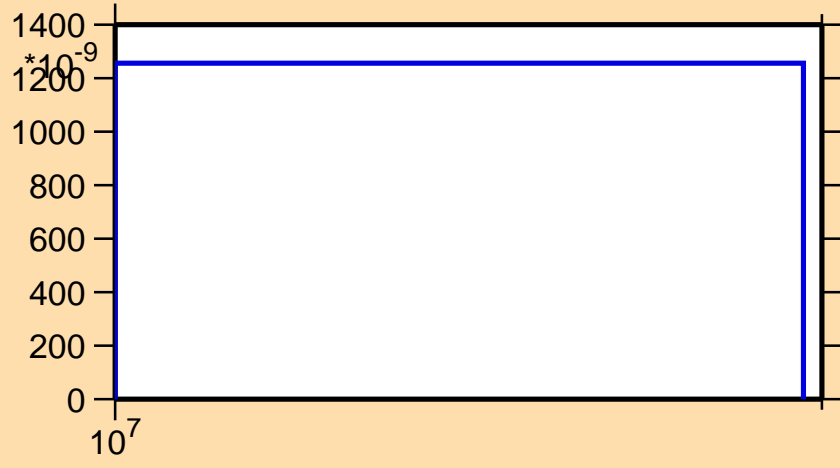
\sigma vs. E for ^{97}\text{Y}(n,nt)
