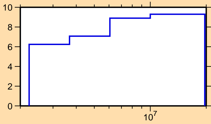
\Delta\sigma/\sigma vs. E for ^{97}\text{Y}(n,n\text{onel.})
