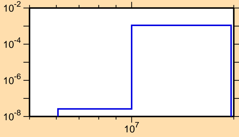
\sigma vs. E for ^{97}\text{Y}(n,p)
