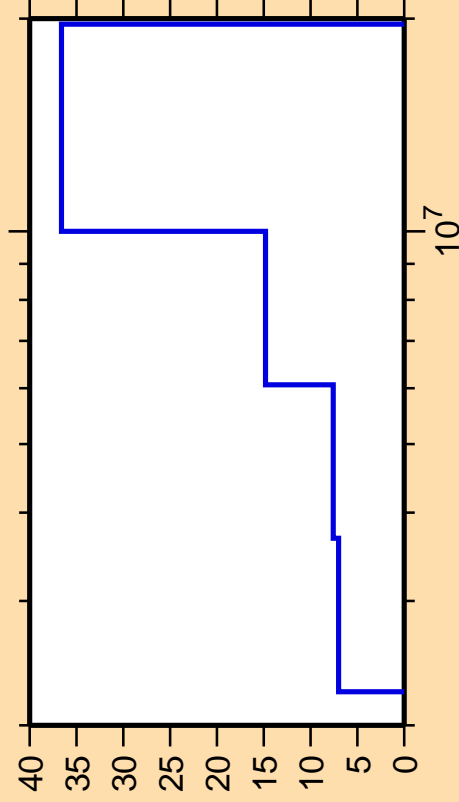
\Delta\sigma/\sigma vs. E for ^{97}\text{Y}(n,ncont.)
