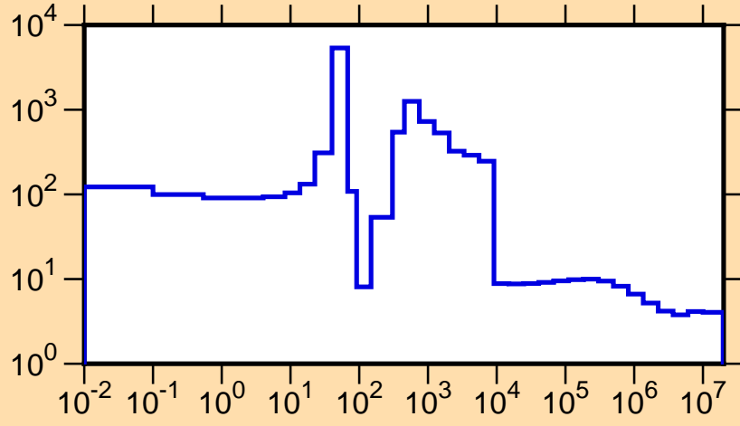
\sigma vs. E for ^{97}\text{Y}(n,\text{tot.})
