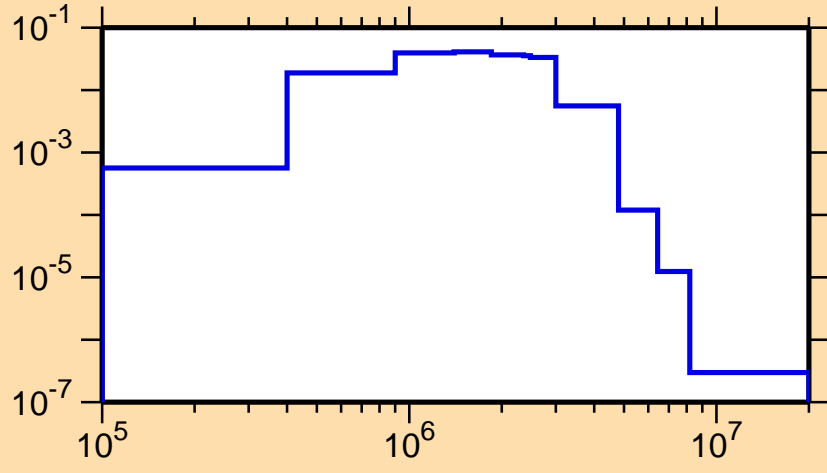
\sigma vs. E for ^{97}\text{Y}(n,n_3)
