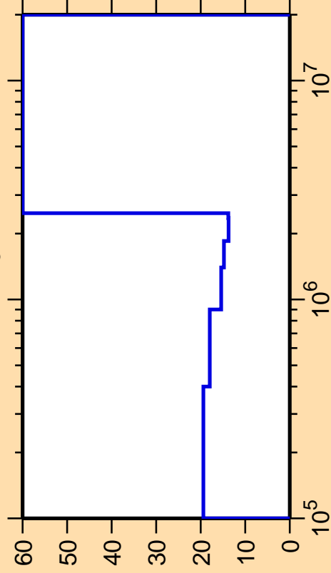
\Delta\sigma/\sigma vs. E for ^{97}\text{Y}(n,n_3)
