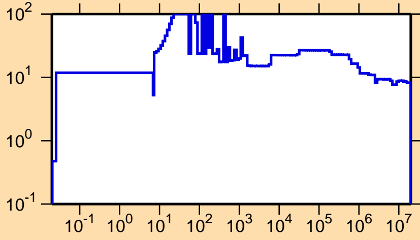
\Delta\sigma/\sigma vs. E for ^{98}\text{Y}(n,\text{nonel.})
