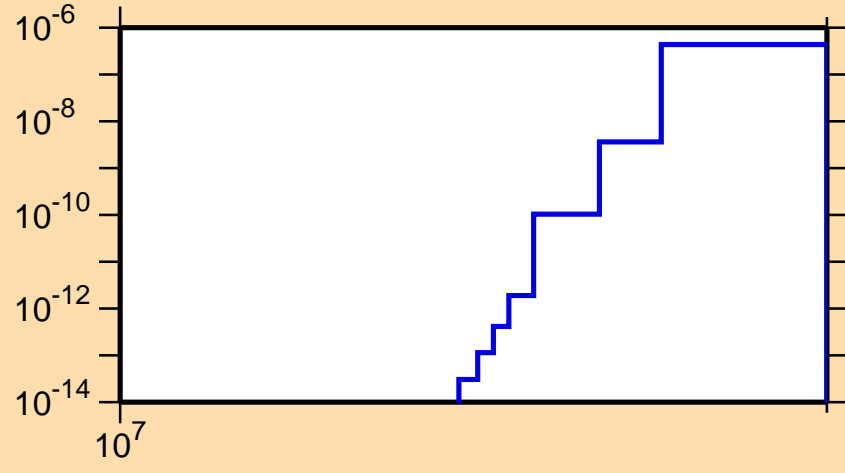
\sigma vs. E for ^{98}\text{Y}(n,2n\alpha)
