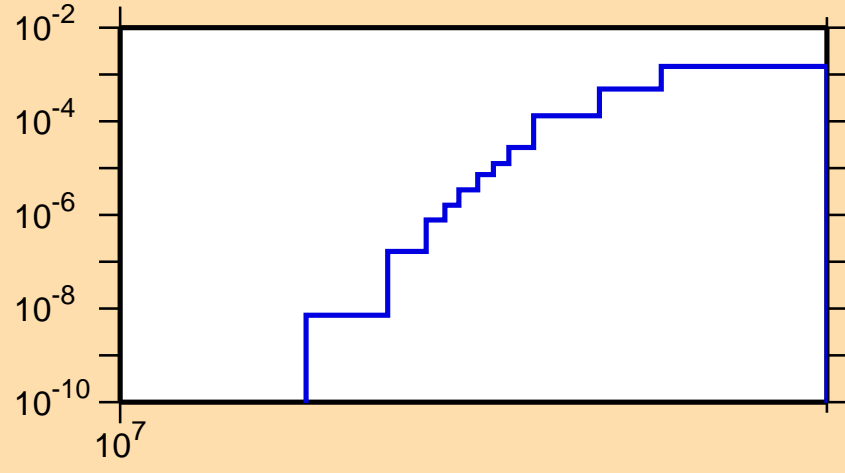
\sigma vs. E for ^{98}\text{Y}(n,np)
