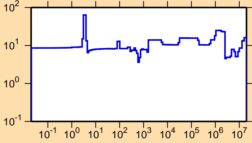
\Delta\sigma/\sigma vs. E for ^{98}\text{Y}(n,\text{el.})
