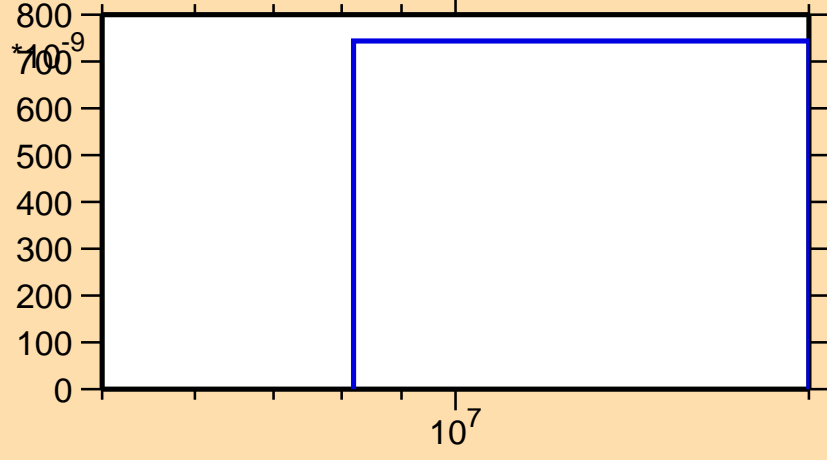
\sigma vs. E for ^{98}\text{Y}(n,\text{nd})
