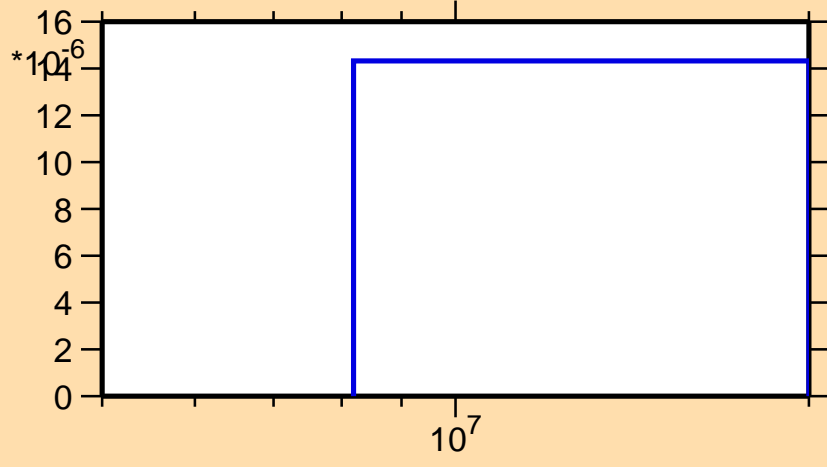
\sigma vs. E for ^{98}\text{Y}(n,n\alpha)
