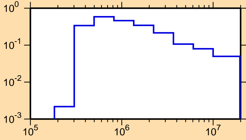
\sigma vs. E for ^{99}\text{Y}(n,n_2)
