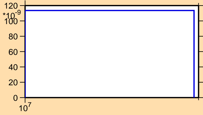
\sigma vs. E for ^{99}\text{Y}(n,nt)
