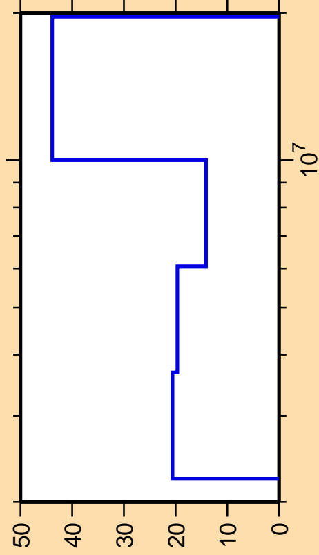
\Delta\sigma/\sigma vs. E for ^{99}\text{Y}(n,n\text{cont.})
