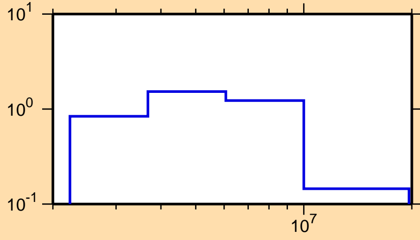
\sigma vs. E for ^{99}\text{Y}(n,n\text{cont.})
