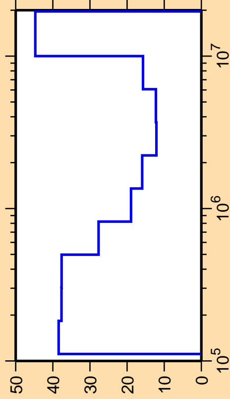
\Delta\sigma/\sigma vs. E for ^{99}\text{Y}(n,\text{inel.})
