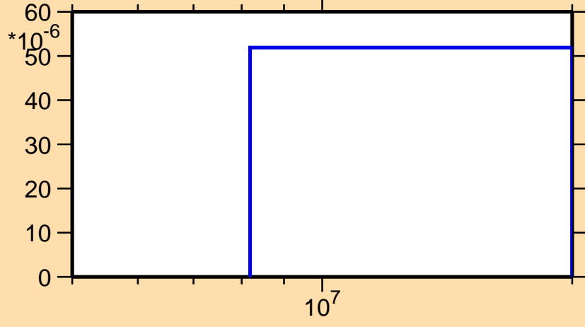
\sigma vs. E for ^{99}\text{Y}(n,d)
