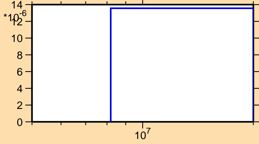
\sigma vs. E for ^{99}\text{Y}(n,\alpha)
