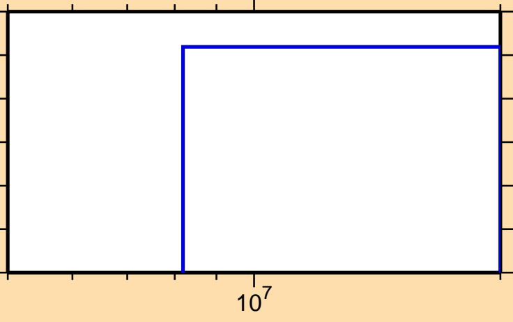
\sigma vs. E for ^{99}\text{Y}(n,d)
