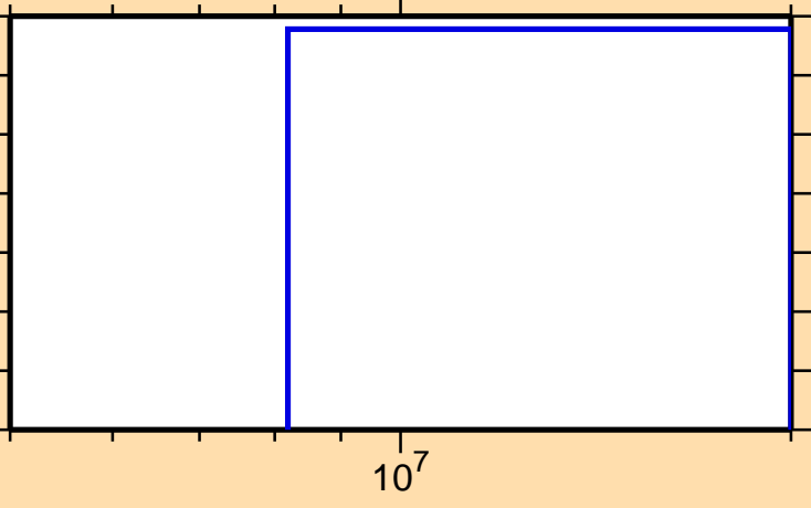
\sigma vs. E for ^{99}\text{Y}(n,\alpha)
