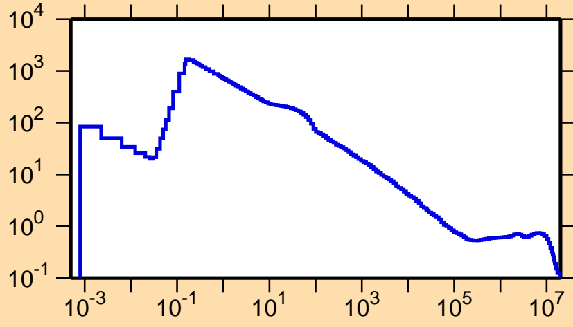
\sigma vs. E for ^{155}\text{Yb}(n,p)
