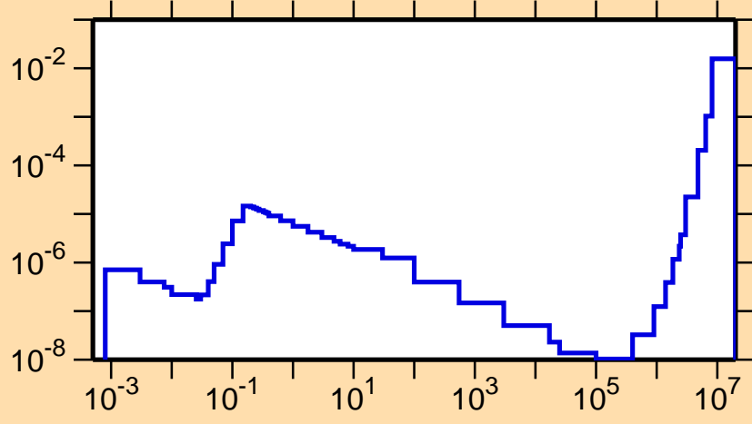
\sigma vs. E for ^{155}\text{Yb}(n,p\alpha)
