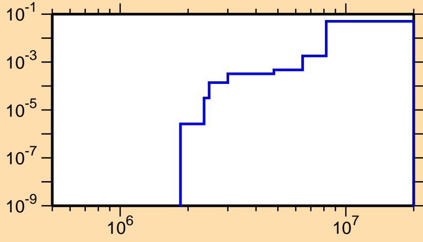
\sigma vs. E for ^{155}\text{Yb}(n,n\alpha)
