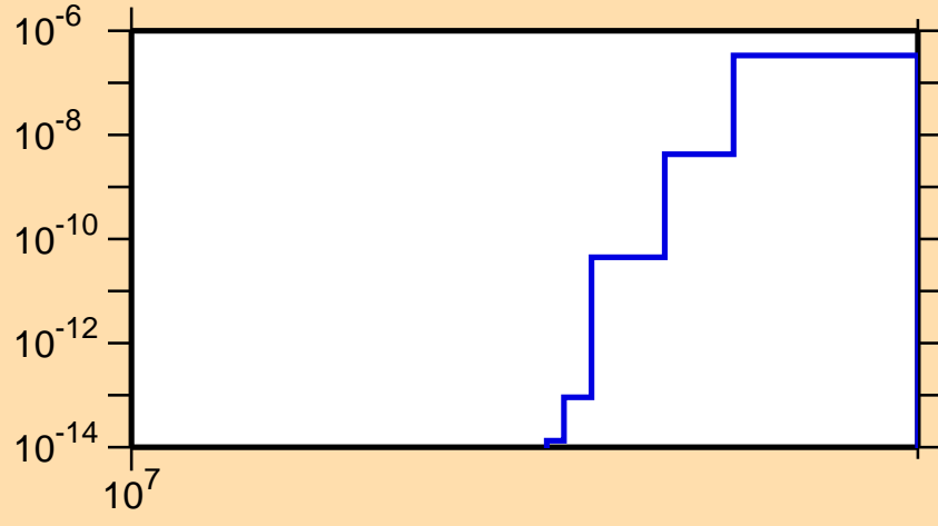
\sigma vs. E for ^{156}\text{Yb}(n,nd)
