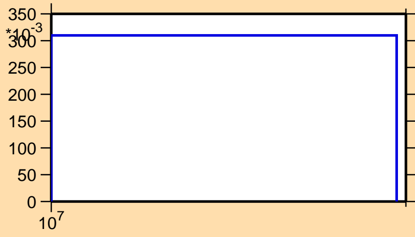
\sigma vs. E for ^{156}\text{Yb}(n,2n)
