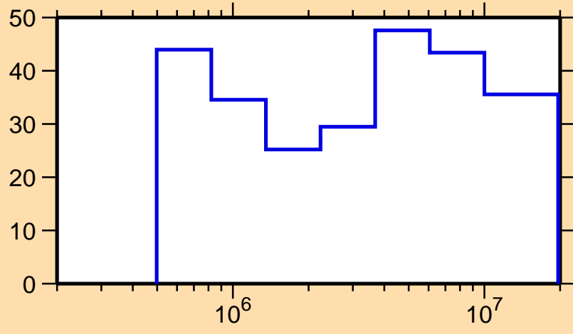
\Delta\sigma/\sigma vs. E for ^{156}\text{Yb}(n,\text{inel.})
