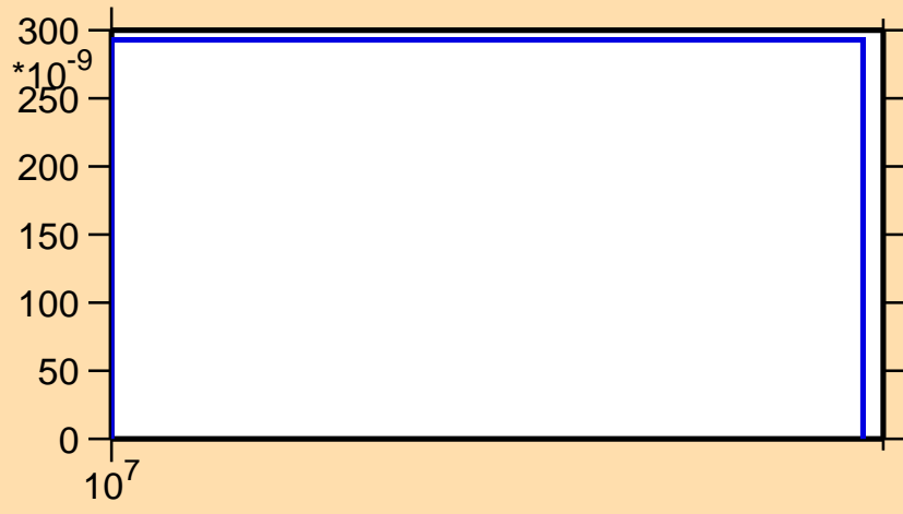
\sigma vs. E for ^{156}\text{Yb}(n,2np)
