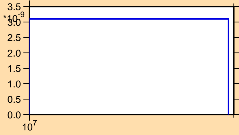
\sigma vs. E for ^{156}\text{Yb}(n,\text{nd})
