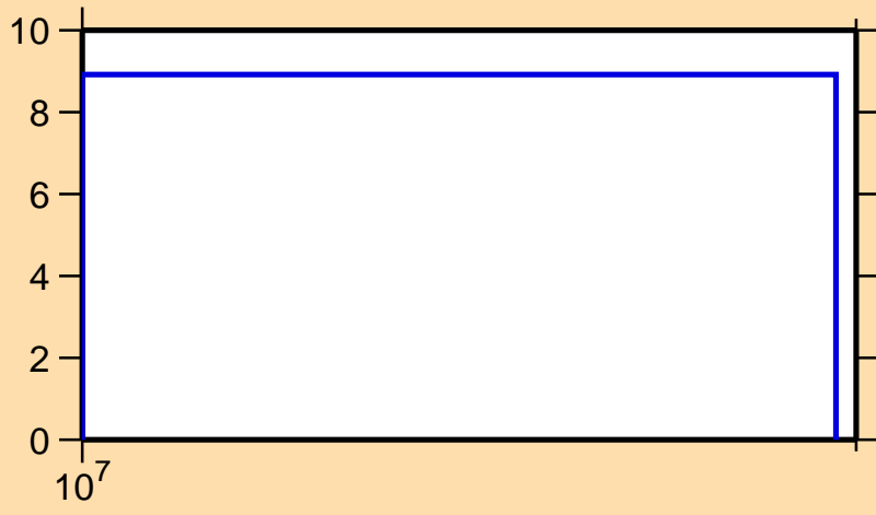
\Delta\sigma/\sigma vs. E for ^{156}\text{Yb}(n,\text{nonel.})
