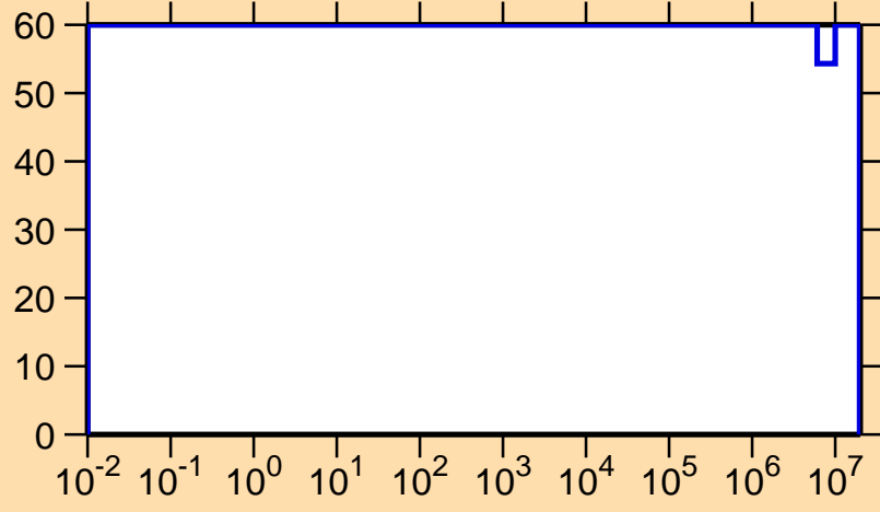
\Delta\sigma/\sigma vs. E for ^{156}\text{Yb}(n,p)
