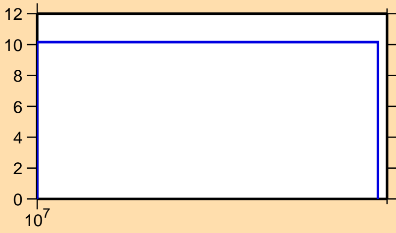
\Delta\sigma/\sigma vs. E for ^{156}\text{Yb}(n,\text{el.})
