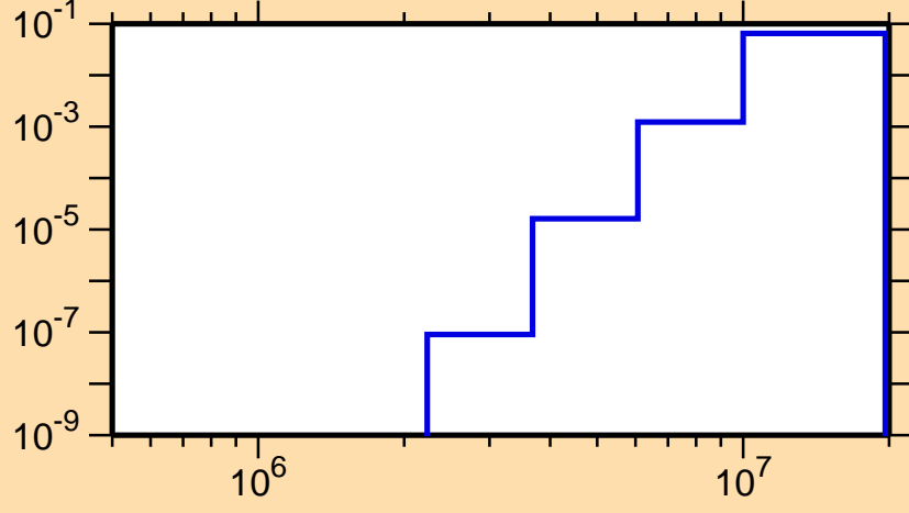
\sigma vs. E for ^{156}\text{Yb}(n,n\alpha)
