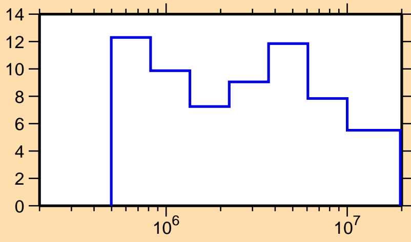
\Delta\sigma/\sigma vs. E for ^{156}\text{Yb}(n,\text{tot.})
