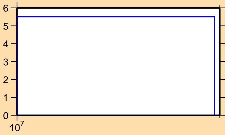
\Delta\sigma/\sigma vs. E for ^{156}\text{Yb}(n,\text{tot.})
