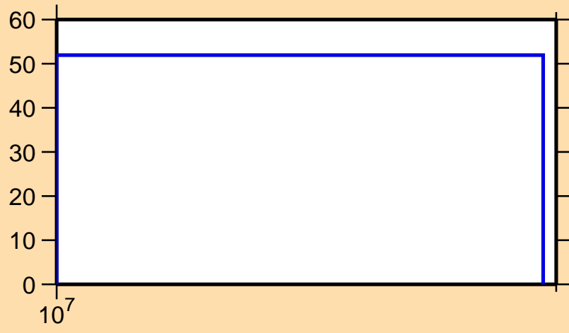
\Delta\sigma/\sigma vs. E for ^{156}\text{Yb}(n,2n)
