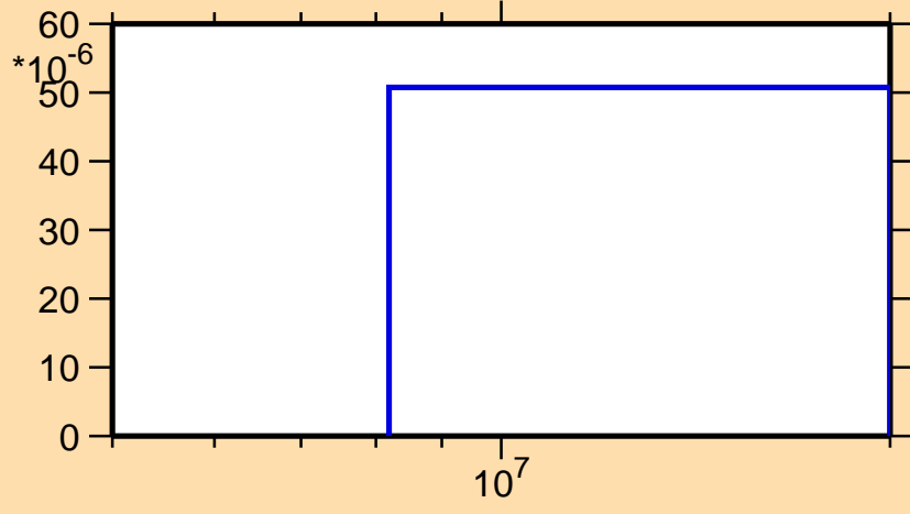
\sigma vs. E for ^{156}\text{Yb}(n,t)
