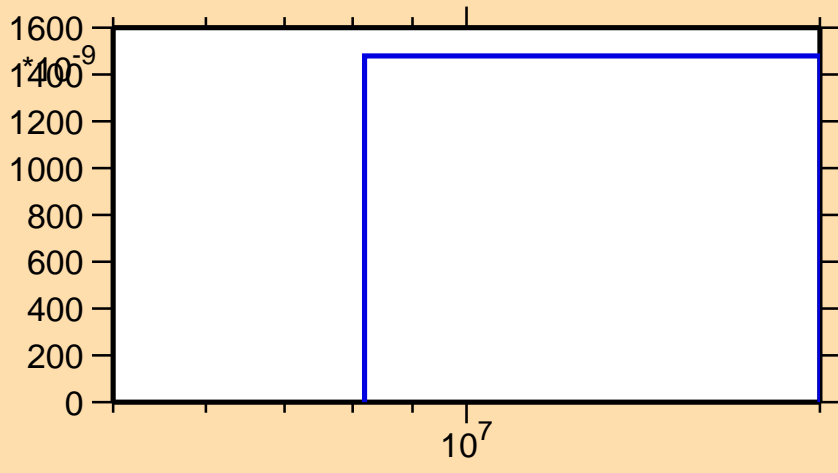
\sigma vs. E for ^{156}\text{Yb}(n,\text{pd})
