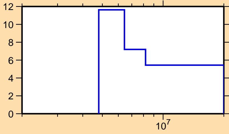
\Delta\sigma/\sigma vs. E for ^{156}\text{Yb}(n, tot.)
