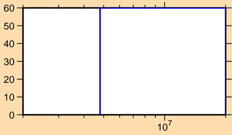
\Delta\sigma/\sigma vs. E for ^{156}\text{Yb}(n,n\text{cont.})
