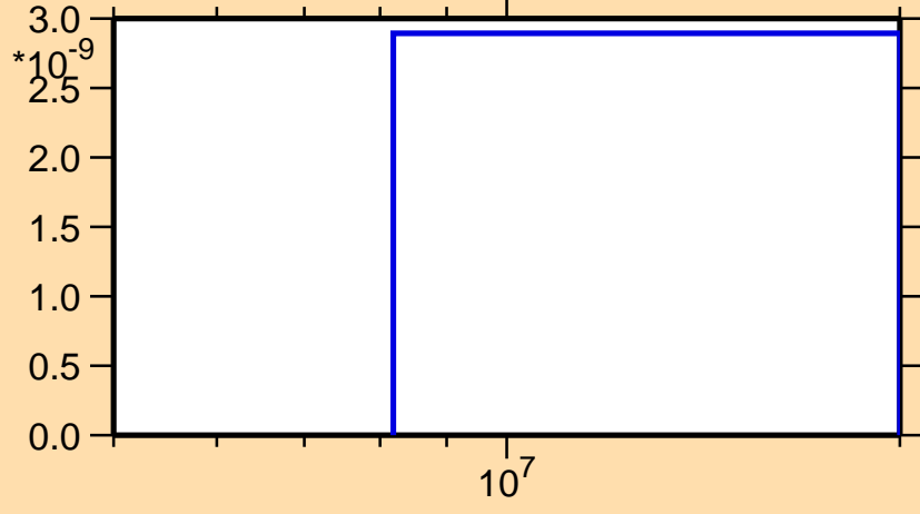
\sigma vs. E for ^{156}\text{Yb}(n,\text{nd})
