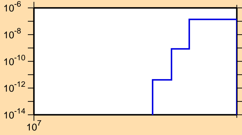
\sigma vs. E for ^{158}\text{Yb}(n,\text{nd})
