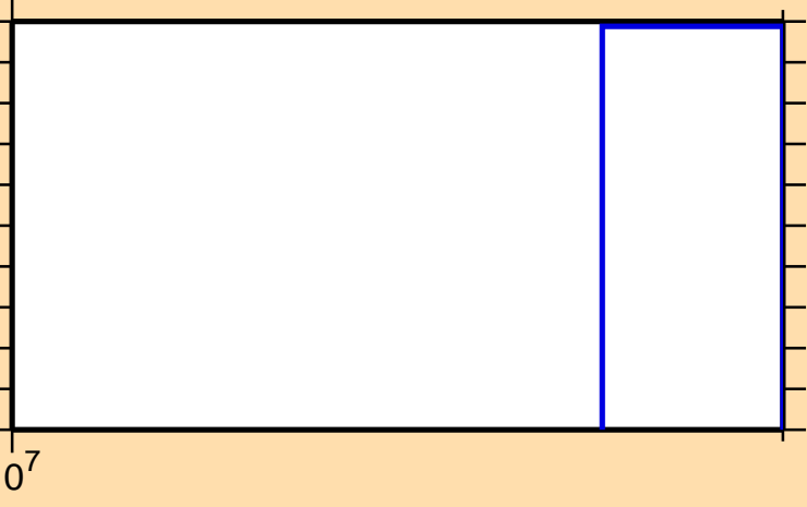
\sigma vs. E for ^{158}\text{Yb}(n,3n)
