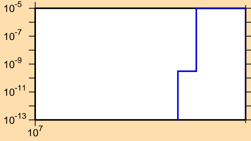
\sigma vs. E for ^{158}\text{Yb}(n,2np)
