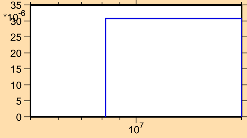
\sigma vs. E for ^{158}\text{Yb}(n,t)
