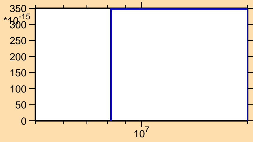
\sigma vs. E for ^{158}\text{Yb}(n,nt)
