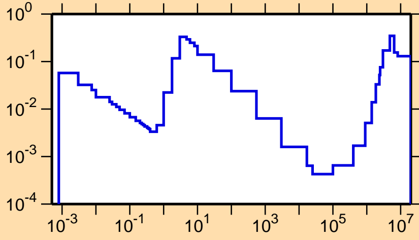
\sigma vs. E for ^{158}\text{Yb}(n,p)
