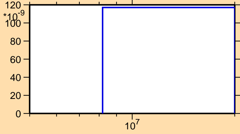
\sigma vs. E for ^{158}\text{Yb}(n,\text{pd})
