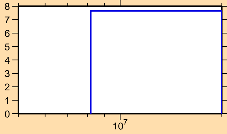
\Delta\sigma/\sigma vs. E for ^{158}\text{Yb}(n,\text{el.})
