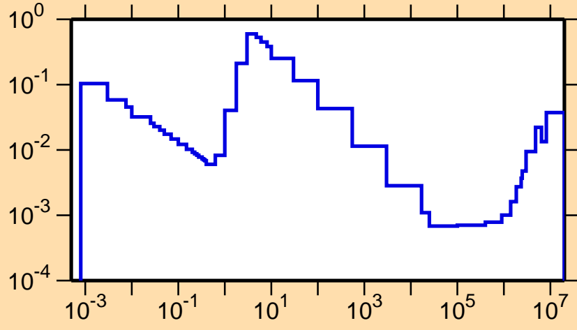
\sigma vs. E for ^{158}\text{Yb}(n,\alpha)
