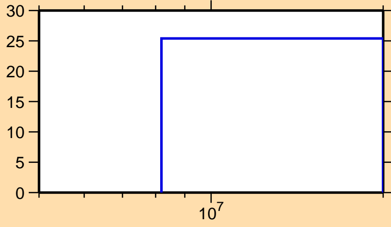
\Delta\sigma/\sigma vs. E for ^{158}\text{Yb}(n,\text{inel.})
