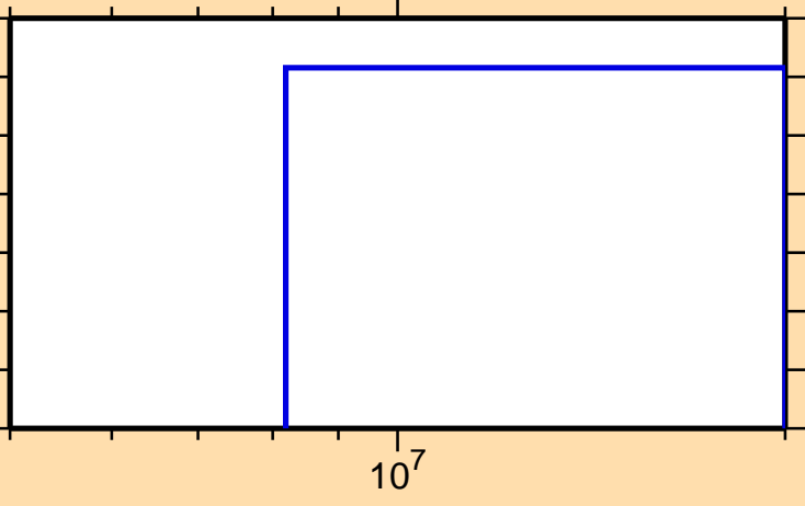
\sigma vs. E for ^{158}\text{Yb}(n,t)
