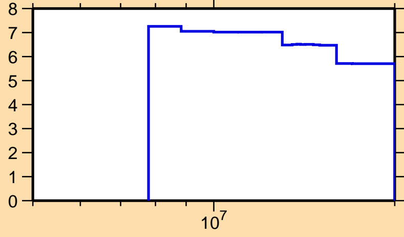
\Delta\sigma/\sigma vs. E for ^{159}\text{Yb}(n,\text{nonel.})
