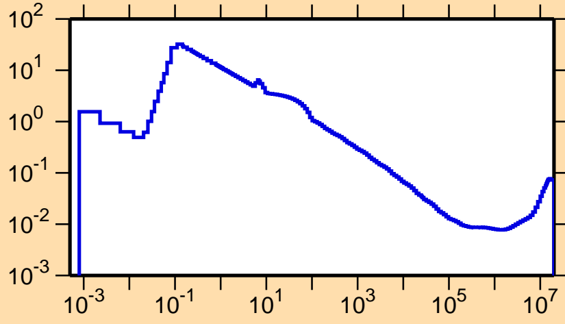
\sigma vs. E for ^{159}\text{Yb}(n,\alpha)
