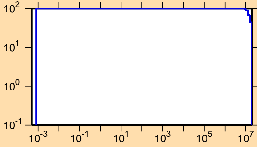
\Delta\sigma/\sigma vs. E for ^{159}\text{Yb}(n,p)
