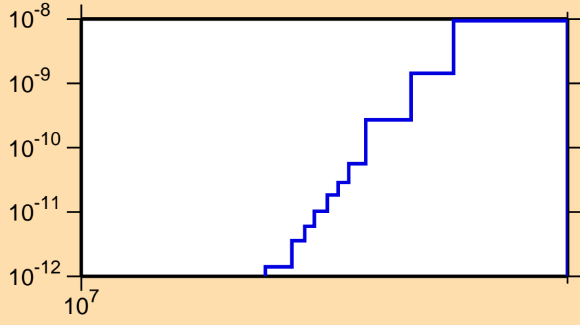
\sigma vs. E for ^{159}\text{Yb}(\text{mt117})
