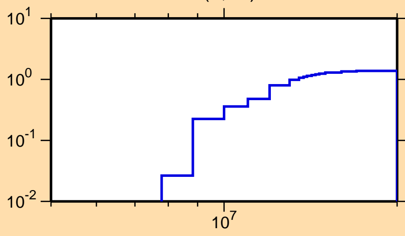
\sigma vs. E for ^{159}\text{Yb}(n,2n)
