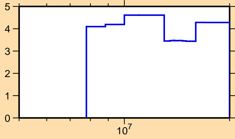
\Delta\sigma/\sigma vs. E for ^{159}\text{Yb}(n,\text{tot.})
