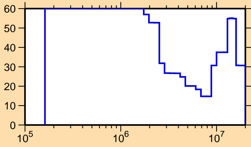
\Delta\sigma/\sigma vs. E for ^{159}\text{Yb}(n,n\text{cont.})
