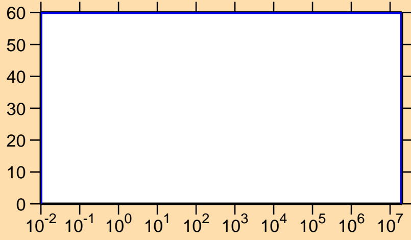
\Delta\sigma/\sigma vs. E for ^{159}\text{Yb}(n,p)
