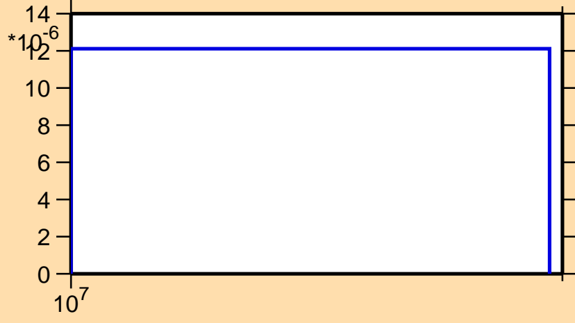
\sigma vs. E for ^{159}\text{Yb}(n,2np)
