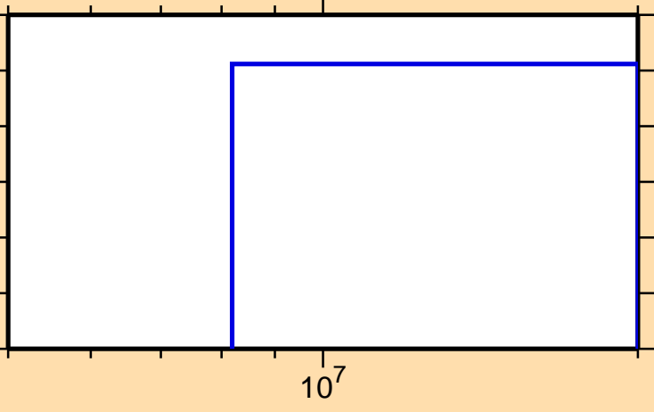
\sigma vs. E for ^{159}\text{Yb}(n,2np)
