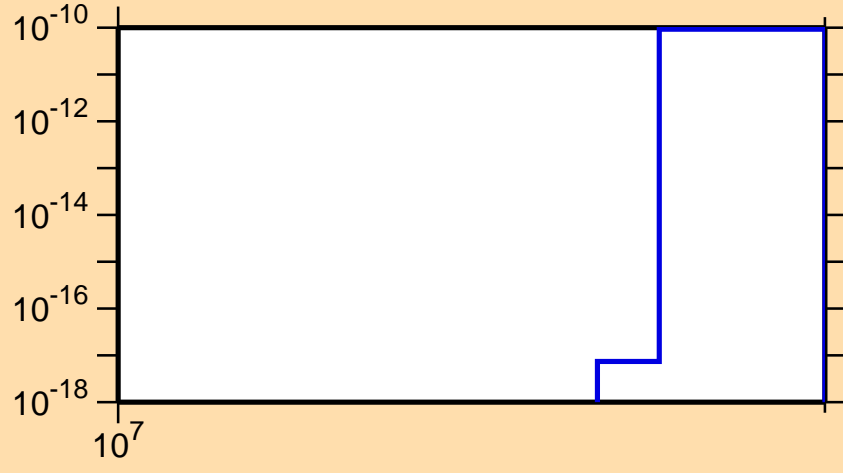
\sigma vs. E for ^{162}\text{Yb}(n,nt)
