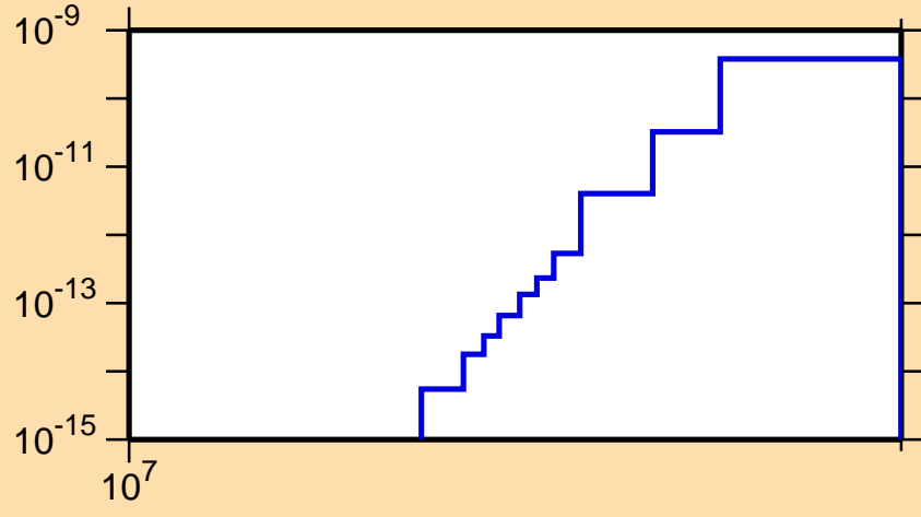
\sigma vs. E for ^{162}\text{Yb}(\text{mt117})
