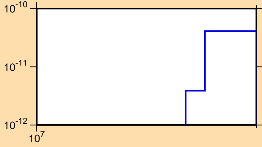
\sigma vs. E for ^{163}\text{Yb}(\text{mt117})
