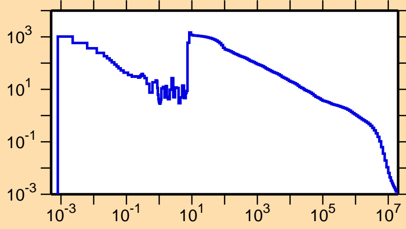
\sigma vs. E for ^{163}\text{Yb}(n,\gamma)
